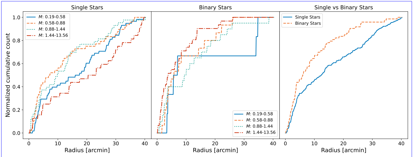
Fig. 9. Left panel: The cumulative distributions of single stars within NGC 6383 are segmented into four mass quartiles ranging from 0.19\text{--}0.58 M_{\odot} to 1.44\text{--}13.56 M_{\odot} , illustrating the spatial distribution across different mass ranges and highlighting the potential influences of mass on the distribution of stars within the cluster. Middle panel: The same distributions as in the left panel for binary stars only, where binaries are defined as sources with a binary probability of at least 0.6. Right panel: The normalized cumulative distributions compare single stars with binary stars, with masses between 0.19 M_{\odot} and 13.56 M_{\odot} . All plots are based on stars with a membership pseudo-probability of at least 0.6. The corresponding KS test results are given in Sect. 7.
