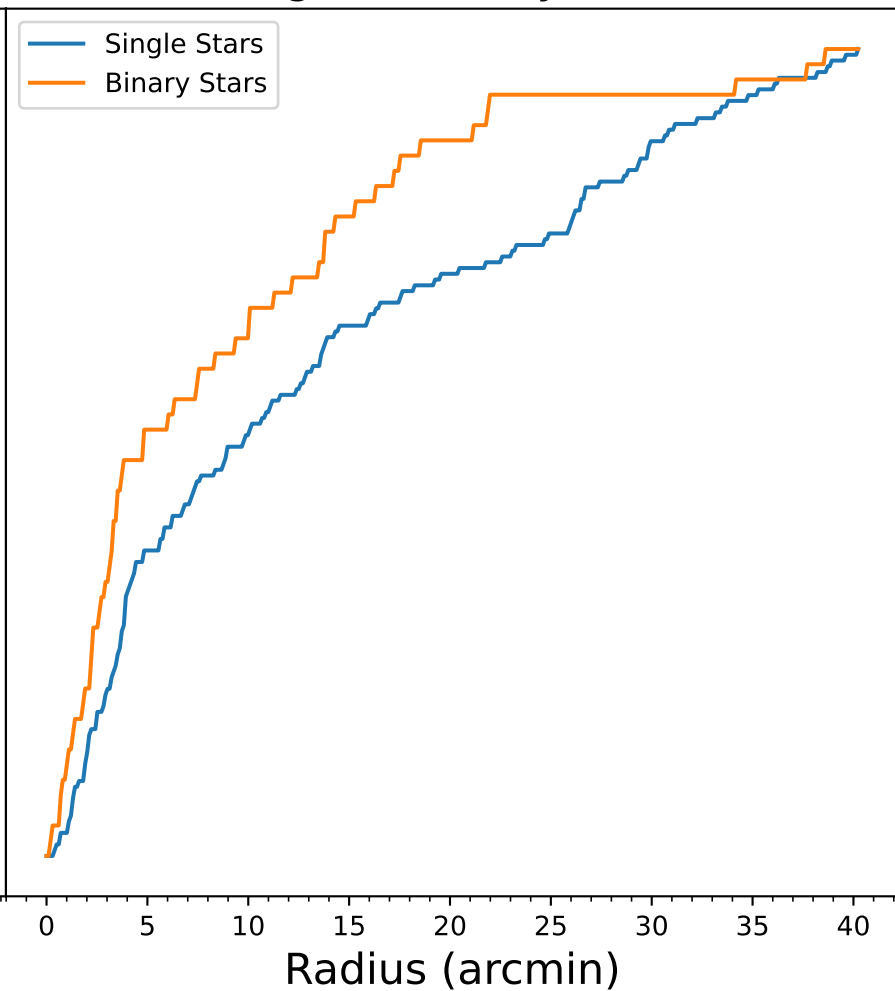
Single vs Binary Stars
