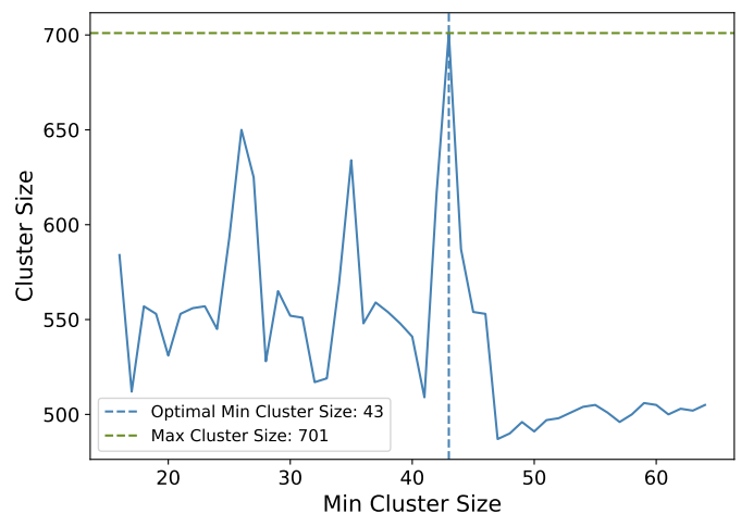
Fig. B.1. Cluster size variation as a function of minimum cluster size, determined through HDBSCAN clustering on the proper-motion data of the sources. The blue line represents shows the recovered cluster sizes achieved at various minimum cluster sizes. The size; the dashed blue line highlights marks the optimal adopted minimum cluster size of 43, where the cluster size reaches a peak. The peaks, and the dashed green line indicates the maximum observed cluster size of 701. Only sweep runs passing in the branch-stability criteria stable regime (condensed-tree \lambda_{max} \geq 8 and recovered branch size between 200 and 701 of 200–701 sources) are shown, which is why the axis does not span the full m_{cl} = 10 –299 grid; this display cut does not enter the selection of m_{cl} .
