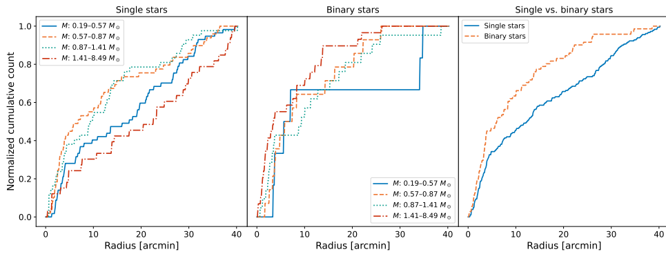
Fig. C.5. Same as Fig. 9, but restricted to stars whose segregation time exceeds the cluster age ( t_{\text{seg}}(m) > 3.53 Myr, i.e., m < 9.1 M_\odot ; Sect. 7); the mass quartiles are recomputed for this truncated sample (uppermost quartile 1.41–8.49 M_\odot ).
