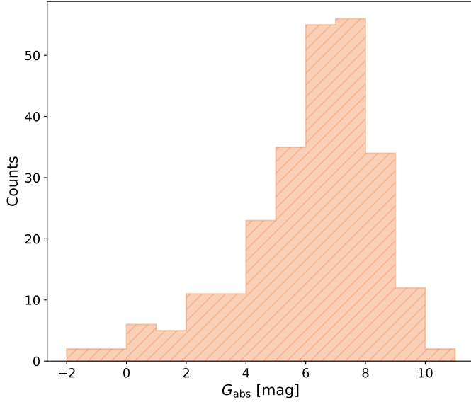
Fig. C.2. Luminosity function of NGC 6383: histogram (orange, hatched) of absolute magnitudes ( G_{abs} ) for stars with a membership pseudo-probability of at least 0.6.
