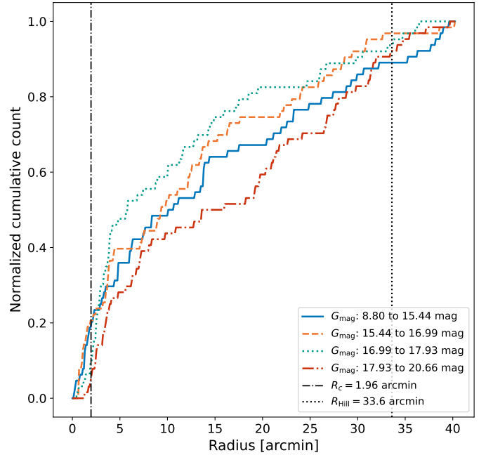
Fig. 8. Normalized cumulative counts of reference-sample stars ( \bar{p} \geq 0.6 ) versus distance from the cluster center, in four G_{\text{mag}} quartiles whose ranges are given in the legend. The black dash-dotted and black dotted vertical lines mark the core radius R_c = 1.96 arcmin and the Hill radius R_{\text{Hill}} = 33.6 arcmin; the adopted King outer radius, R_t = 54^{+7}_{-11} arcmin (Appendix D), lies beyond the plotted range of this 40 arcmin sample.
