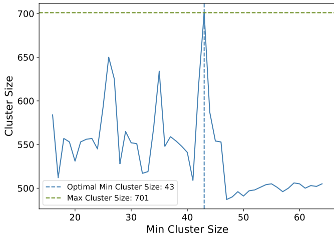
Fig. B.1. Cluster size variation as a function of minimum cluster size, determined through HDBSCAN clustering on the proper-motion data of the sources. The blue line shows the recovered cluster size; the dashed blue line marks the adopted minimum cluster size of 43, where the cluster size peaks, and the dashed green line the maximum observed cluster size of 701. Only sweep runs in the stable regime ( \lambda_{\max} \geq 8 and recovered branch of 200–701 sources) are shown, which is why the axis does not span the full m_{\text{cl}} = 10 –299 grid; this display cut does not enter the selection of m_{\text{cl}} .
