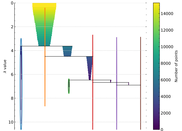
Fig. B.2. Condensed cluster tree (dendrogram) from the HDBSCAN analysis: NGC 6383 cluster sources on the left, HDBSCAN-identified field sources on the right. Branch width and color give the number of sources at each level (color bar); \lambda = 1/d_{\text{mreach}} is the inverse mutual-reachability distance. Colored ellipses mark the leaf clusters selected by HDBSCAN; the tall blue ellipse on the left, persisting over the widest \lambda range, is the branch adopted as NGC 6383.
