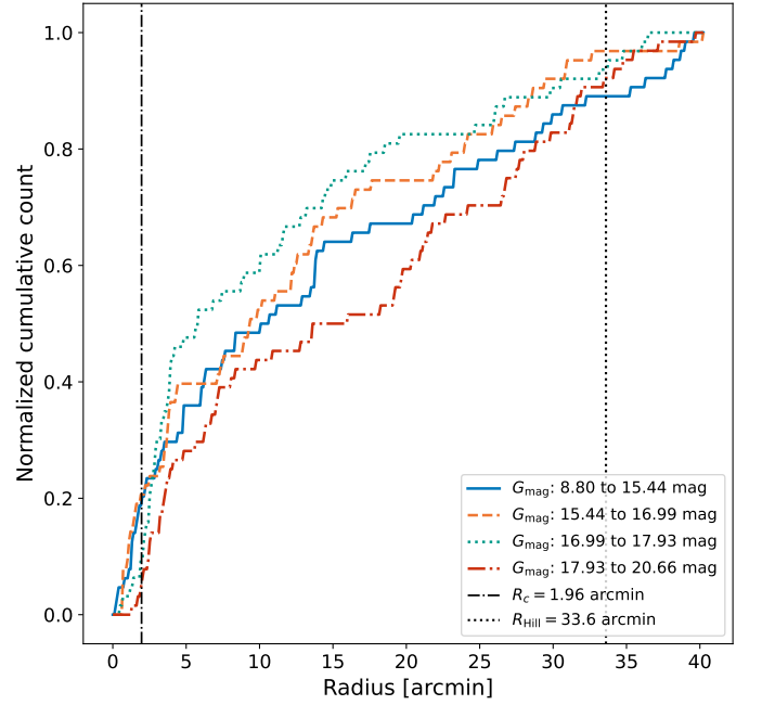
Fig. 8. Normalized cumulative counts of reference-sample stars ( \bar{p} \geq 0.6 ) within NGC 6383 are plotted against radial distance from the cluster center for different brightness ranges, segmented into quartiles of G_{\text{mag}} , whose ranges are given in the legend. The black dash-dotted and black dotted vertical lines mark the core radius R_c = 1.96 arcmin and the Hill radius R_{\text{Hill}} = 33.6 arcmin; the adopted King outer radius, R_t = 54^{+7}_{-11} arcmin (Appendix D), lies beyond the plotted range of this 40 arcmin sample.
