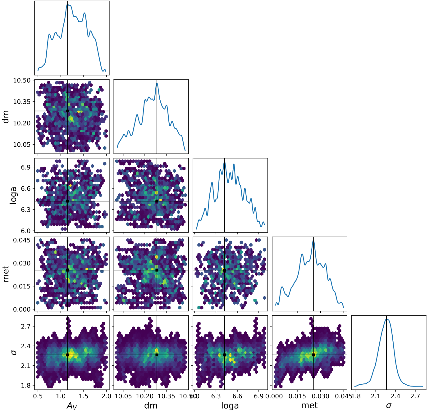
Fig. B.4. Marginal and joint distributions of the parameters A_V (visual extinction, for a fixed R_V = 3.1 ), dm (distance modulus), \log a (logarithmic age), met (metallicity), and the nuisance likelihood-scatter parameter \sigma , sampled with the DEMetropolis ensemble. The diagonals display the marginal distributions for each parameter (blue curves). The off-diagonal hexbin plots show the joint distributions. Black lines mark the mode of each distribution in all panels; in the off-diagonal panels, the joint mode is additionally marked by a black square.
