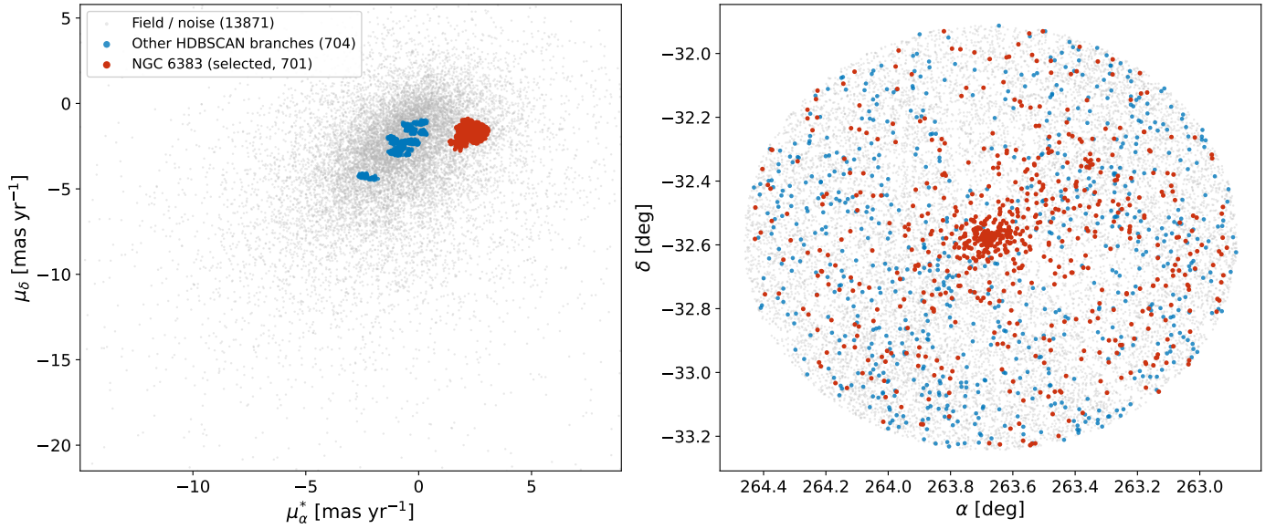
Fig. B.3. Full HDBSCAN clustering panorama of the 40 arcmin preprocessed sample (15276 sources). Left panel: Proper-motion plane ( \mu_\alpha^*, \mu_\delta ). Right panel: On-sky distribution in right ascension and declination. Sources are color-coded by their HDBSCAN label: the selected NGC 6383 branch (red), the other HDBSCAN branches (blue), and the field/noise (gray); the legend lists the number of sources in each group. The proper-motion axes are clipped to the 0.5–99.5 percentile range so that the cluster over-density is visible against the broad field distribution.
