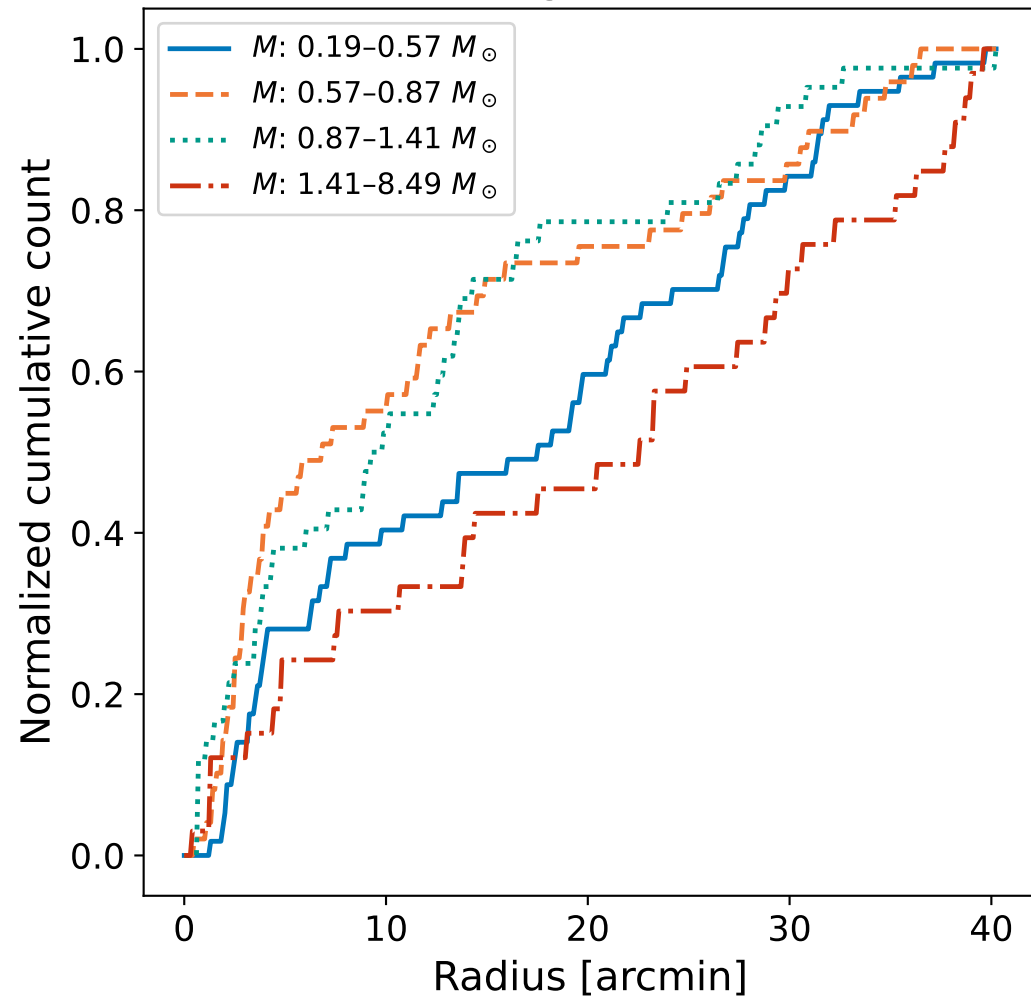
Single stars
