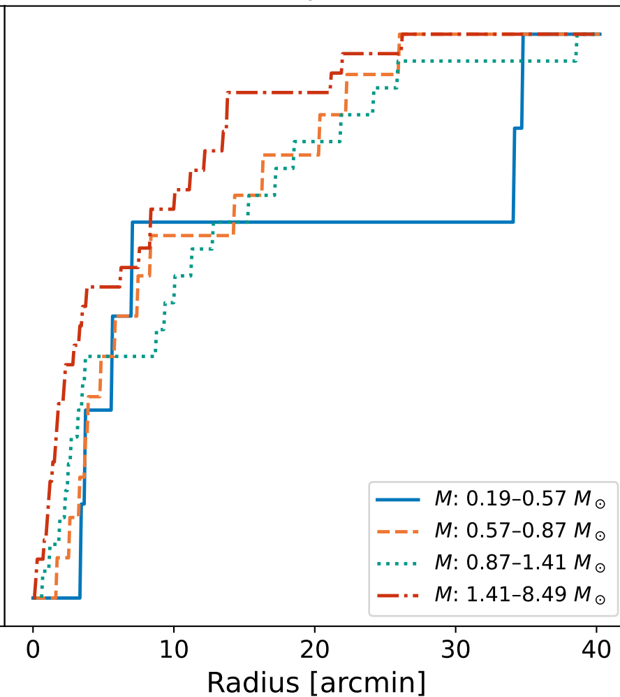
Binary stars
