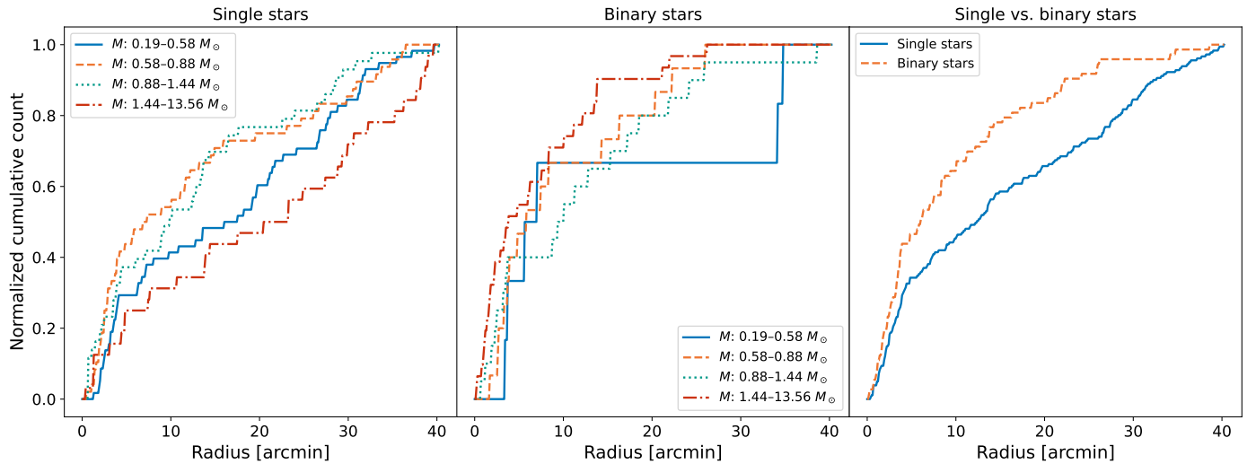
Fig. 9. Left panel: The Radial cumulative distributions of single by mass and binarity. Left panel: Single stars within NGC 6383 are segmented into in four mass quartiles ranging , from 0.19\text{--}0.58 M_{\odot} to 1.44\text{--}13.56 M_{\odot} , illustrating the spatial distribution across different mass ranges and highlighting the potential influences of mass on the distribution of stars within the cluster. Middle panel: The same distributions as in the left panel Same for binary star only, where binaries are defined as sources with a binary probability of at least 0.6. Right panel: The normalized cumulative distributions compare single stars with Single versus binary stars , with masses between 0.19 M_{\odot} and 13.56 M_{\odot} . All plots In the left and middle panels the solid, dashed, dotted, and dash-dotted curves are based on the mass quartiles from lowest to highest; in the right panel single stars are solid and binary stars dashed. All panels use stars with a membership pseudo-probability of at least 0.6. The ; the corresponding KS test results are given in Sect. 7.
