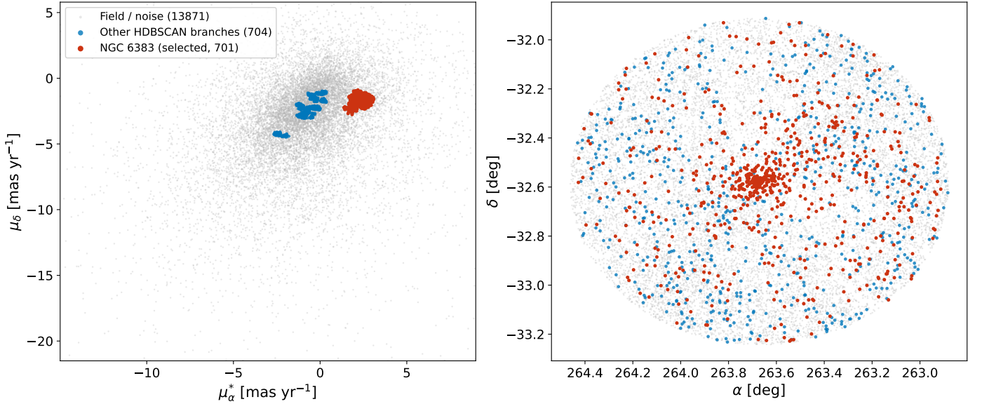
Fig. B.3. Full HDBSCAN clustering panorama of the 40 arcmin preprocessed sample (15276 sources). Left panel: Proper-motion plane ( \mu_\alpha^* , \mu_\delta ). Right panel: On-sky distribution in right ascension and declination. Sources are color-coded by their HDBSCAN label: the selected NGC 6383 branch (red), the other HDBSCAN branches (blue), and the field/noise (gray); the legend lists the number of sources in each group. The proper-motion axes are clipped to the 0.5–99.5 percentile range so that the cluster over-density is visible against the broad field distribution.
