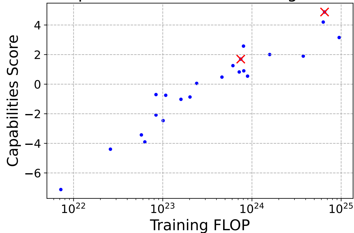
Capabilities Score vs Training FLOP
