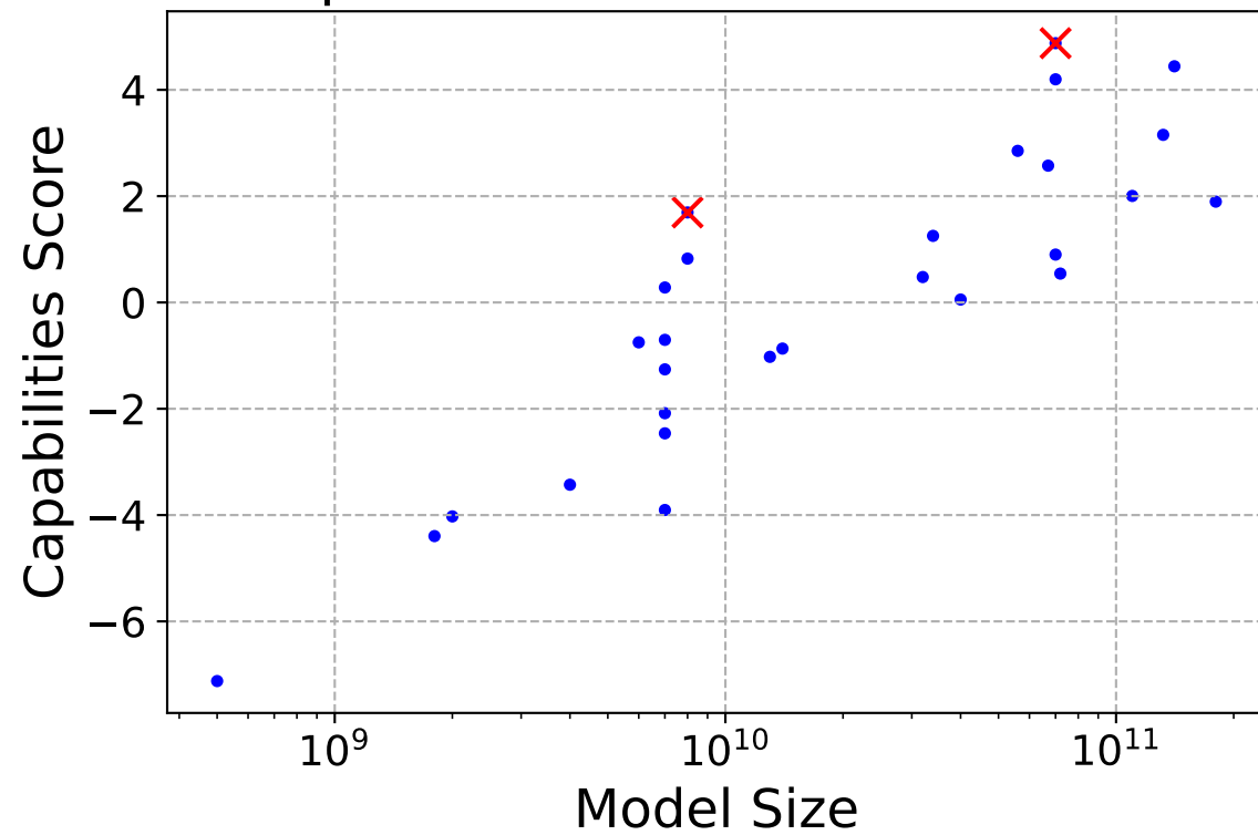
Capabilities Score vs Model Size
