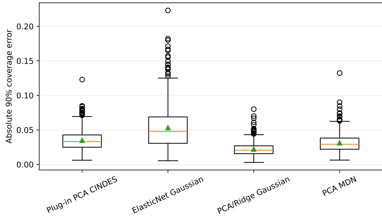
All Eligible Drugs: Coverage Error
