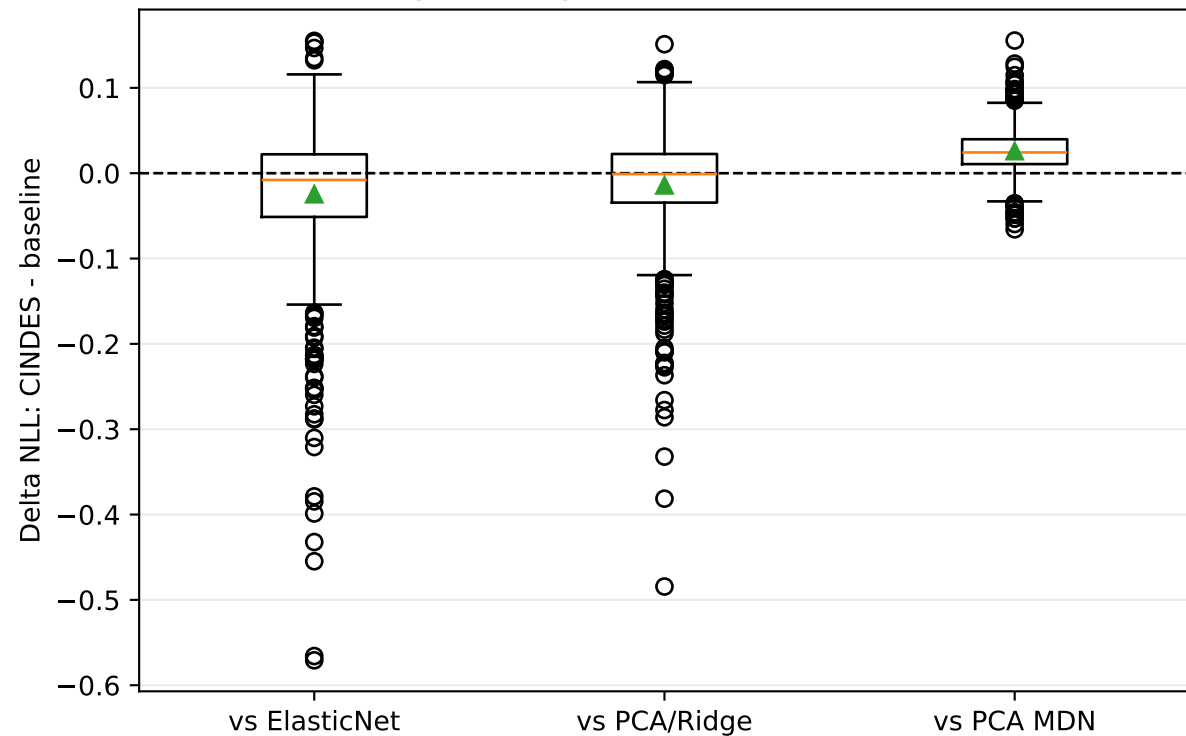
All Eligible Drugs: Pairwise NLL Differences
