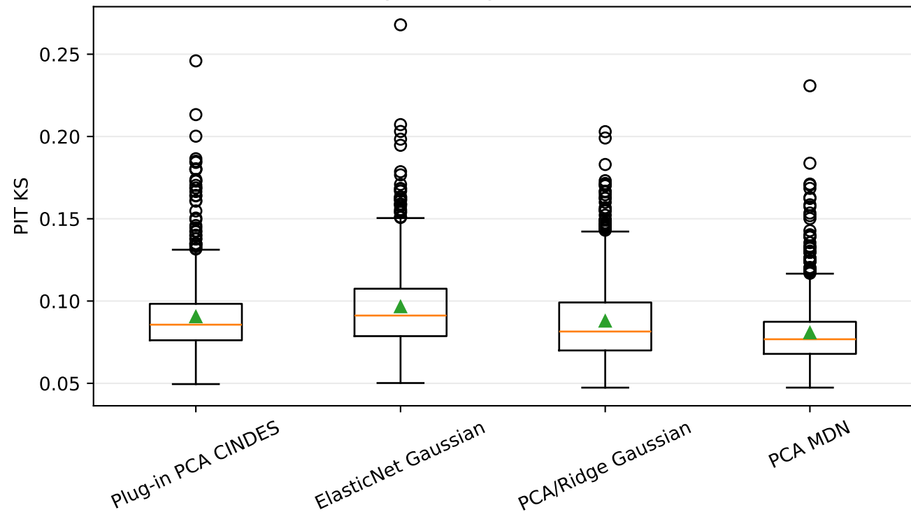
All Eligible Drugs: PIT Calibration
