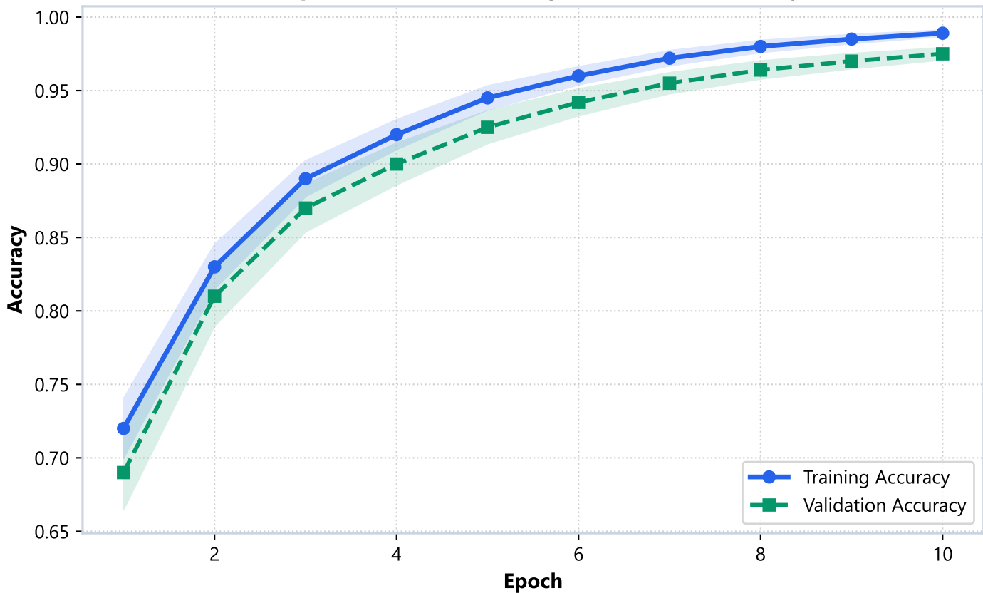
Proposed PM-CNN Training & Validation Accuracy
