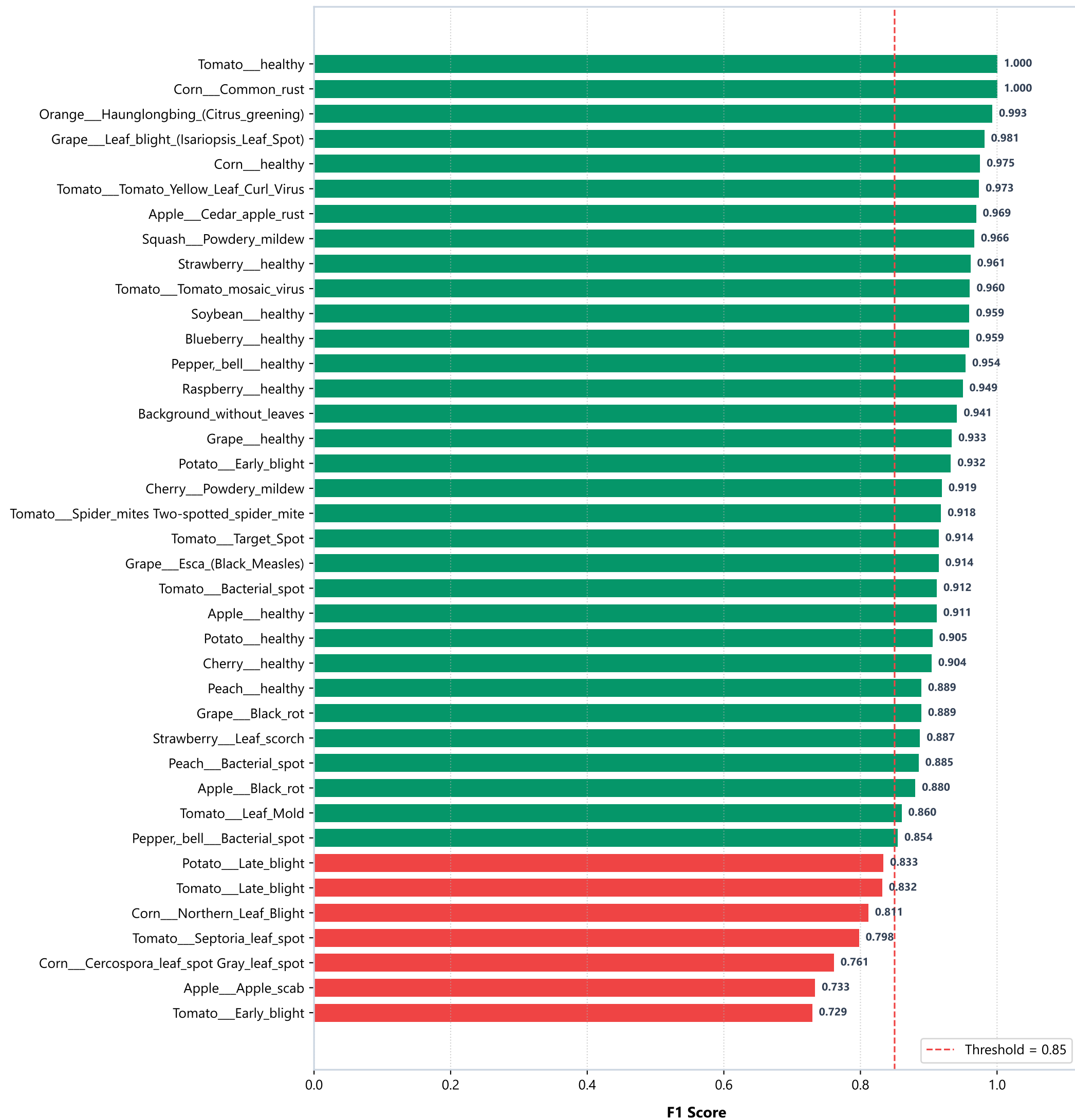
Per-Class F1 Score Performance (Proposed PM-CNN)
