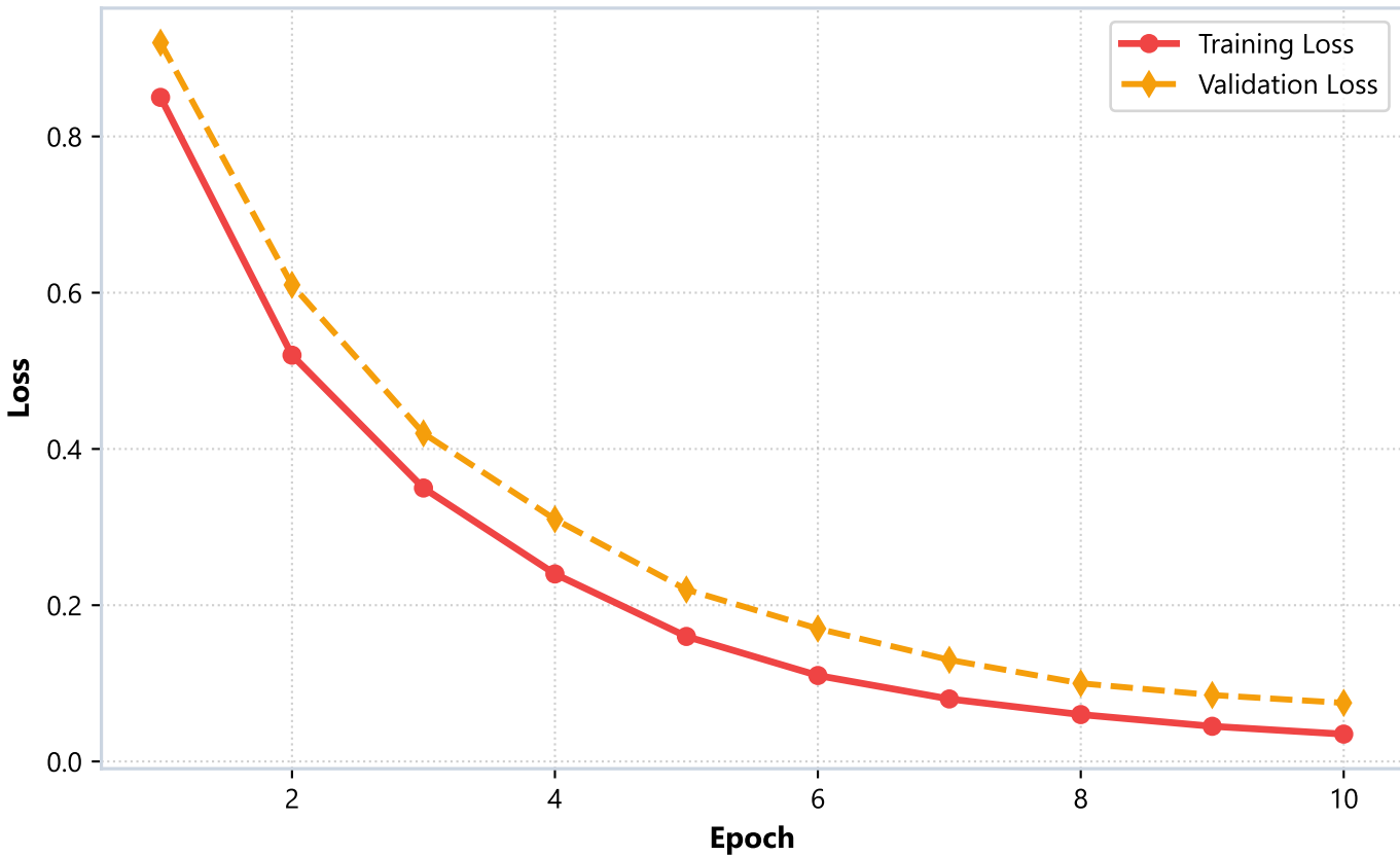
Proposed PM-CNN Training & Validation Loss
