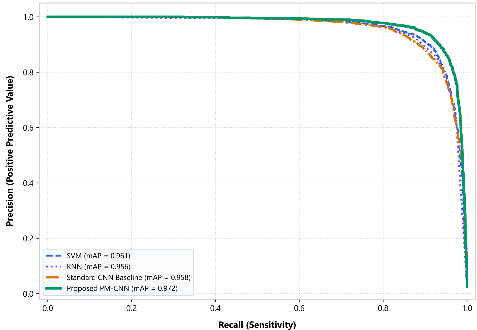
Precision-Recall (PR) Curve 4-Model Comparison
