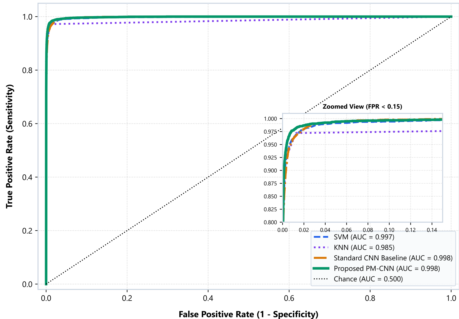
Receiver Operating Characteristic (ROC) 4-Model Comparison
