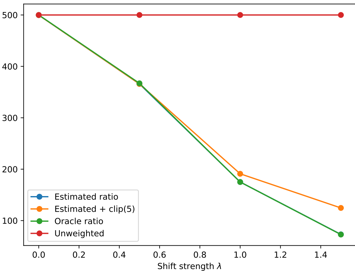
Calibration effective sample size
