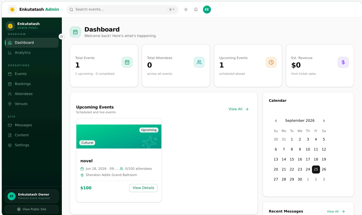
The Dashboard: summary cards on top, upcoming events and calendar below.
