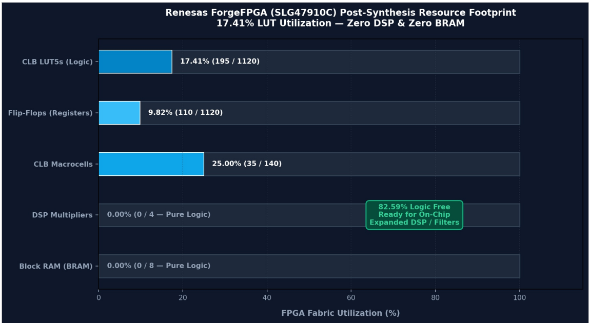
Renesas ForgeFPGA Resource Footprint
