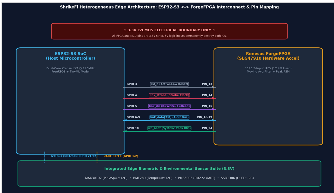
ShrikeFi Pinout & Interconnect Diagram
