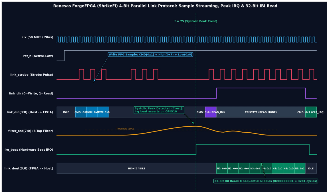
ShrikeFi 4-Bit Parallel Link Protocol Timing Waveform
