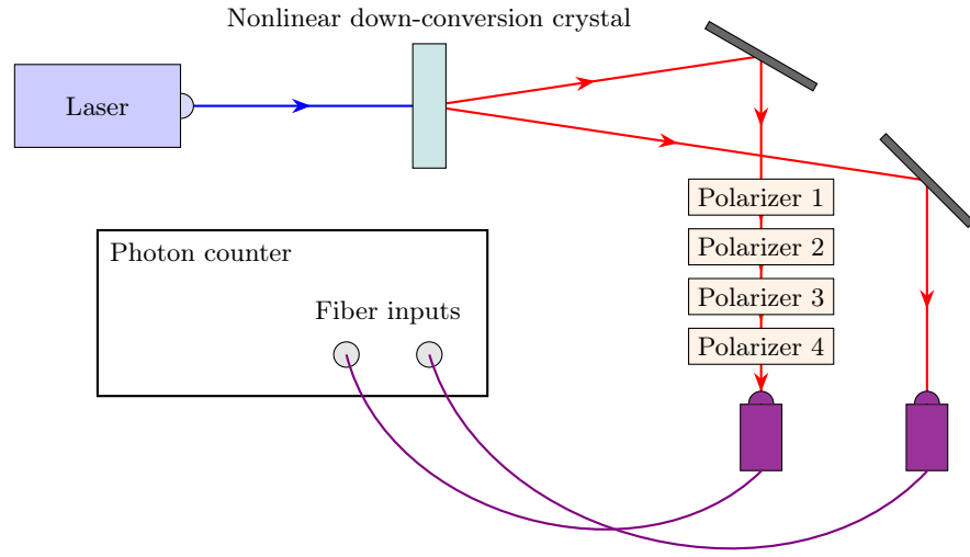
FIG. 1. Experimental setup. The laser diode outputs 405 nm horizontally-polarized light, which passes through a nonlinear down-conversion crystal (beta-barium borate, or BBO), which causes the incident photons to undergo spontaneous parametric down-conversion. This then generates pairs of horizontally-polarized 810 nm photons, which then are separated into two arms. The photon in Arm 0 passes through 4 successive polarizers, whereas the photon in Arm 1 passes through free space. At the end of each arm, the photons are coupled into optical fibers and led into the input of a photon counter that detects coincident photons.
