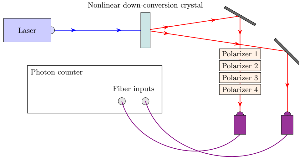
FIG. 1. Experimental setup. The laser diode outputs 405 nm horizontally-polarized light, which passes through a nonlinear down-conversion crystal (beta-barium borate, or BBO), which causes the incident photons to undergo spontaneous parametric down-conversion. This then generates pairs of horizontally-polarized 810 nm photons, which then are separated into two arms. The photon in Arm 0 passes through 4 successive polarizers, whereas the photon in Arm 1 passes through free space. At the end of each arm, the photons are coupled into optical fibers and led into the input of a photon counter that can detect coincident photons.
