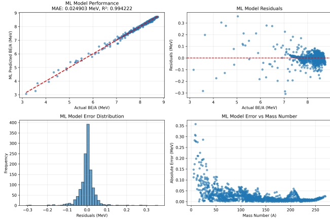
Figure 1: ML Model Validation Results. The four-panel analysis shows (top-left) predicted vs actual binding energy per nucleon with perfect correlation, (top-right) residuals distribution centered around zero, (bottom-left) error distribution histogram, and (bottom-right) error vs mass number showing consistent performance across all nuclear masses. The model achieves 0.025 MeV MAE with R^2 = 0.994 .
