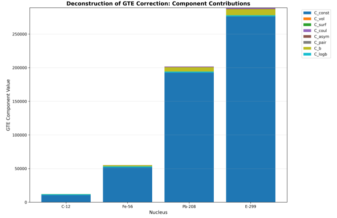
Figure 2: GTE Correction Deconstruction. This analysis breaks down the GTE framework's corrections into their constituent components, showing how different GTE features contribute to the final binding energy predictions. Each component represents a different aspect of the nuclear interaction, demonstrating the framework's ability to capture the complex physics of nuclear binding.
