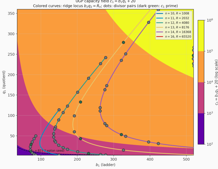
Figure 2: Capacity field c_1 = b_1q_1 + 20 in (b_1, q_1) . Background: log-scaled field; curves: ridge loci b_2q_2 = R_n ; dots: admissible divisor pairs (dark c_1 composite, green c_1 prime). Dashed level: c_1 = 823 (Lepton seed). Right: same field as a surface with ridge curves lifted to height c_1 .
