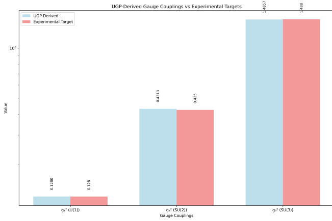
Figure 3: Derived vs. Experimental Gauge Couplings. UGP-derived g_1^2 , g_2^2 , g_3^2 (blue) vs. experimental targets (orange). Artifact: gauge_couplings_comparison.png.
