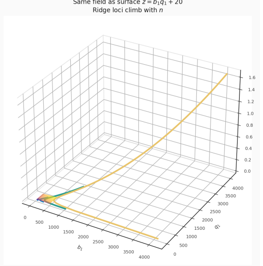
Figure 2: Capacity field c_1 = b_1q_1 + 20 in (b_1, q_1) . Background: log-scaled field; curves: ridge loci b_2q_2 = R_n ; dots: admissible divisor pairs (dark c_1 composite, green c_1 prime). Dashed level: c_1 = 823 (Lepton seed). Right: same field as a surface with ridge curves lifted to height c_1 .
