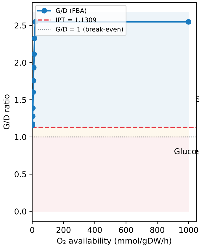
A. Aerobic-anaerobic gradient (glucose, ijO1366 FBA)
