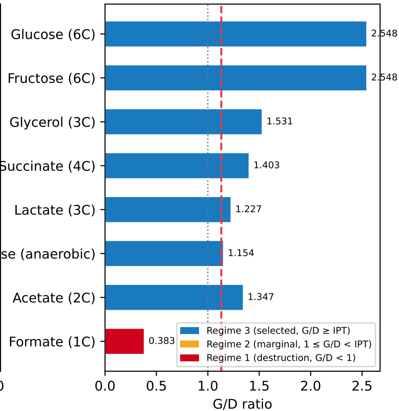
B. Carbon source survey (ijO1366, aerobic/anaerobic)
