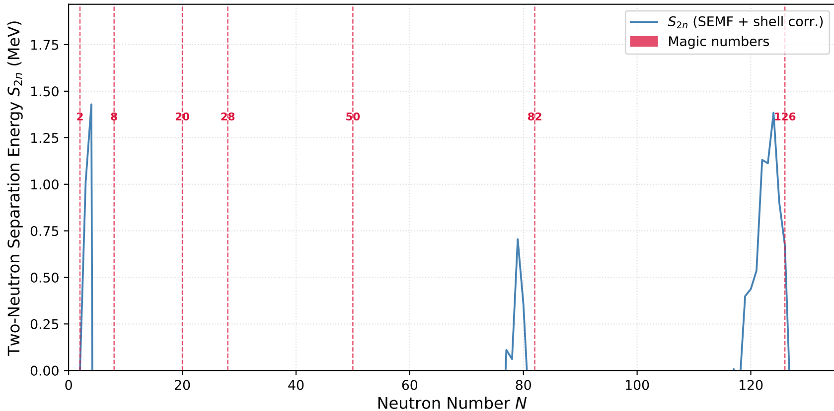
Nuclear Magic Numbers: Anomalous Shell Stability (SEMF + Strutinsky shell correction, \kappa_{\text{emp}} = 0.050 )
