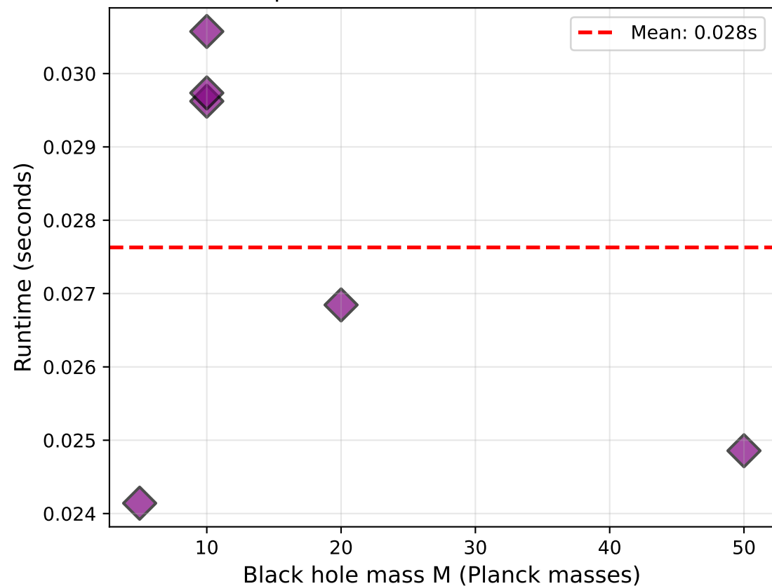
(a) Computational Cost vs. Black Hole Mass
