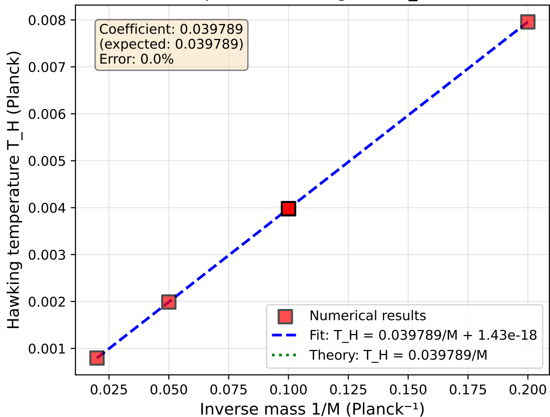
(b) Temperature Scaling Law: T_H \propto 1/M
