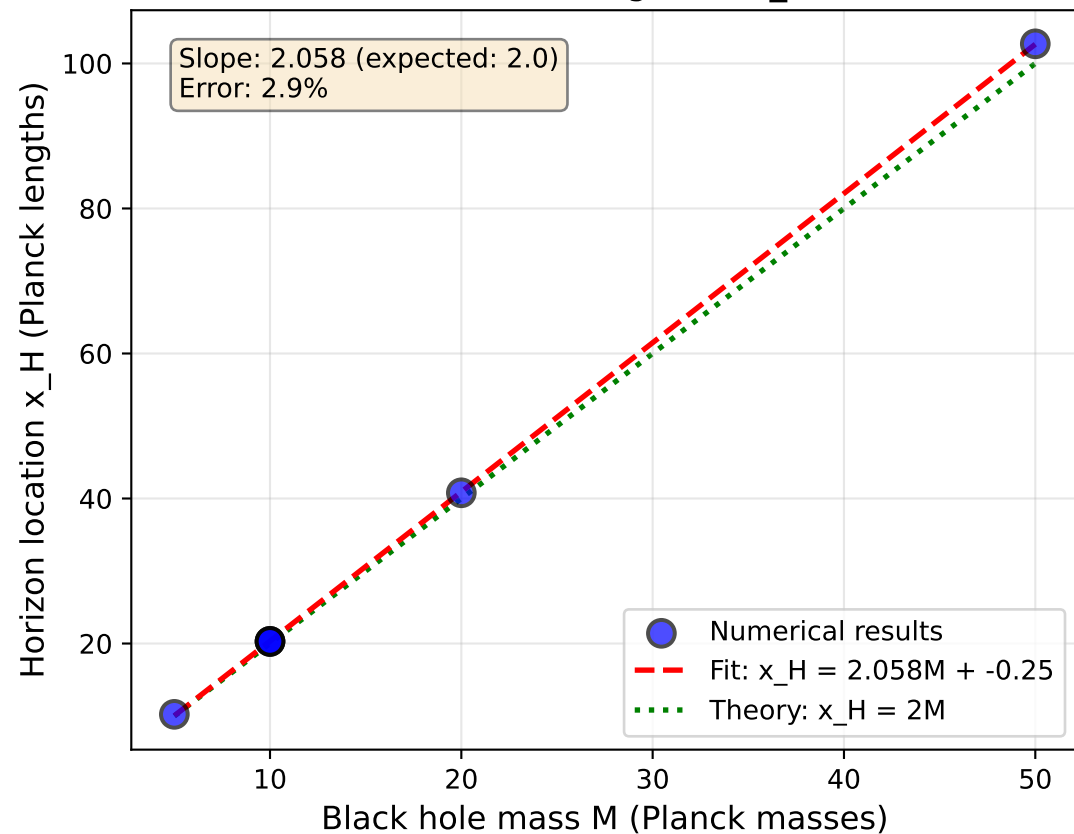
(a) Horizon Scaling Law: x_H \propto M
