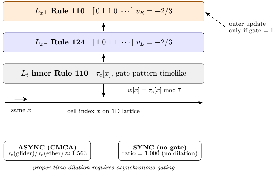
Figure 1: The Chiral Minkowski CA at one lattice site: two decoupled chiral outer layers ( L_{x+} , L_{x-} ) on the same index x , gated by a shared inner Rule 110 clock ( L_t ). Outer layers advance only when the inner gate fires; differential gate rates between glider and ether cells implement dynamics-level SR time dilation.
