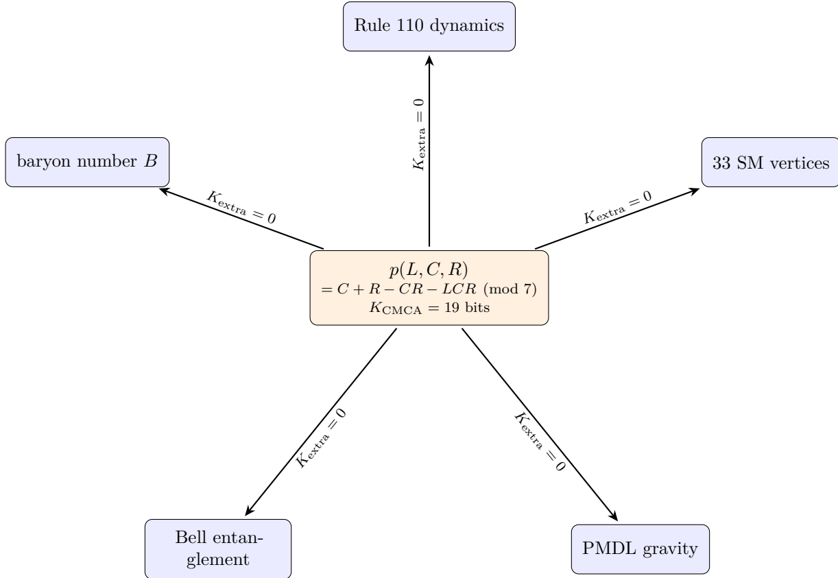
Figure 5.1: The GTE polynomial is a single 19-bit specification whose algebraic structure certifies five independent physical roles with zero additional description length.
