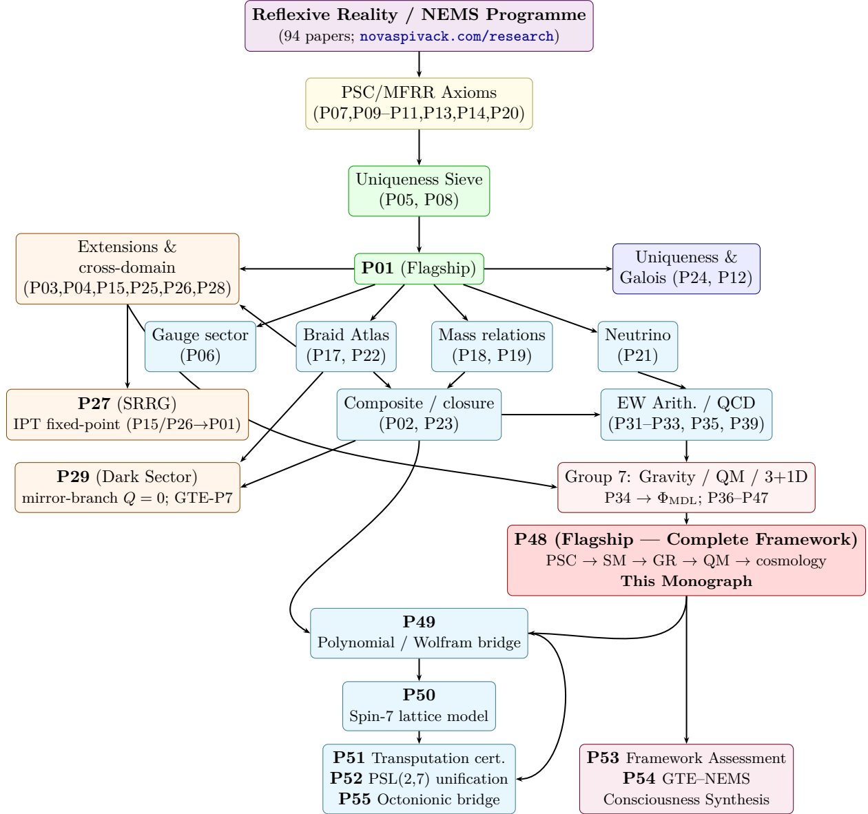
Figure 1.1: Logical dependency structure of the UGP Physics series (P01–P55). Arrows indicate that the target paper depends on results from the source. The purple Group 10 node collects P53 (framework assessment) and P54 (GTE–NEMS consciousness synthesis); both depend on P48.
