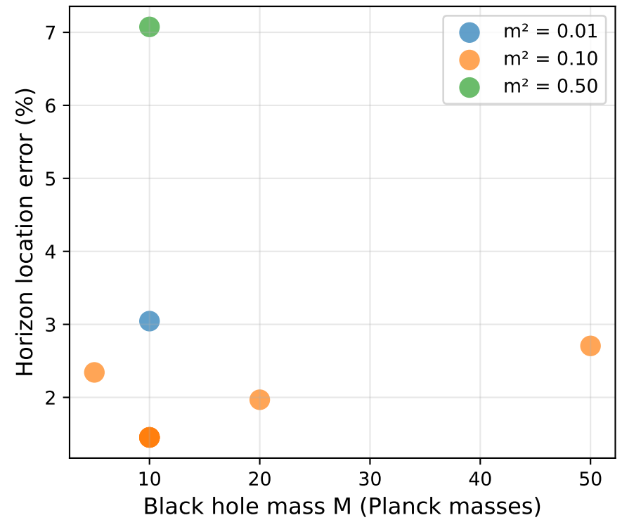
(b) Error vs. Mass & Coherence Field
