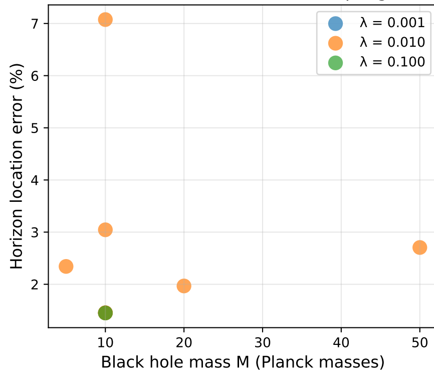
(c) Error vs. Mass & Self-Coupling
