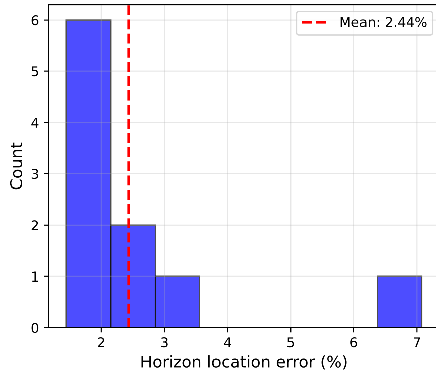
(a) Horizon Location Error Distribution
