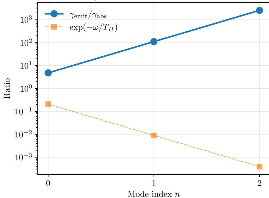
(b) Detailed Balance Check
