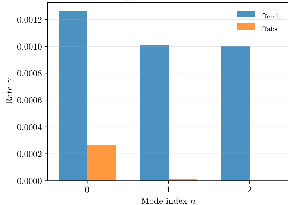
(a) Lindblad Rates
