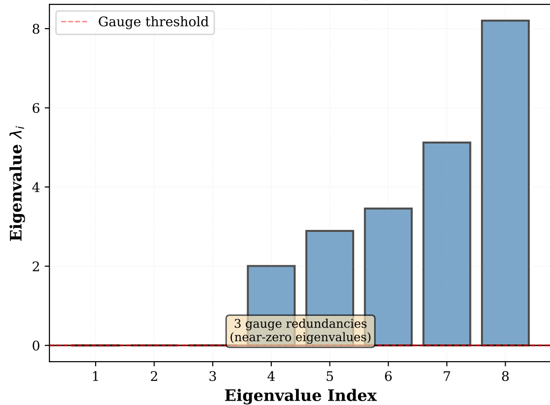
(a) Full 8D Hessian Spectrum
