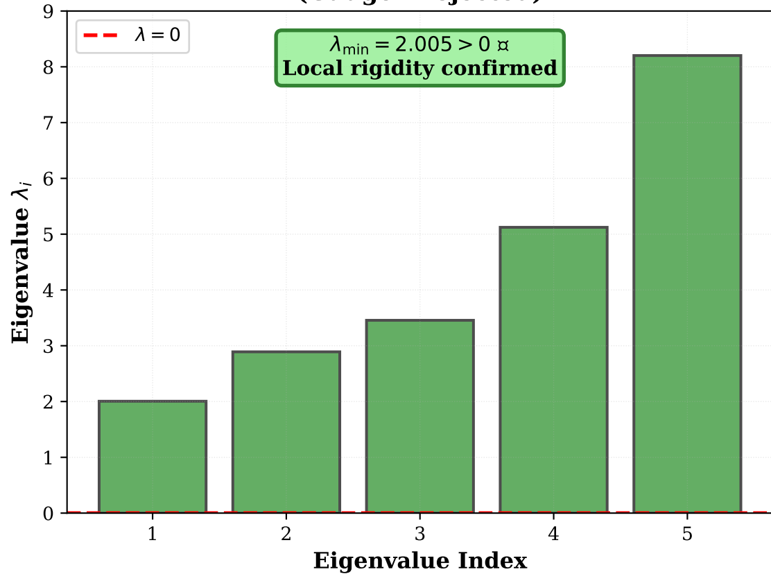
(b) Physical 5D Hessian Spectrum (Gauge-Projected)
