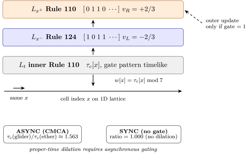
Figure 8.1: The Chiral Minkowski CA at one lattice site: two decoupled chiral outer layers ( L_{x+} , L_{x-} ) on the same index x , gated by a shared inner Rule 110 clock ( L_t ). Outer layers advance only when the inner gate fires; differential gate rates between glider and ether cells implement dynamics-level SR time dilation.
