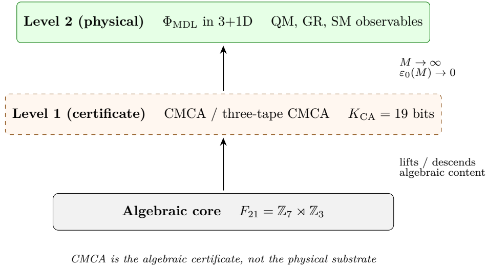
Figure 5.1: \Phi_{\text{MDL}} is the physical field theory; the CMCA is its minimal discrete certificate. Algebraic results propagate in both directions; geometric precision requires the continuum limit.
