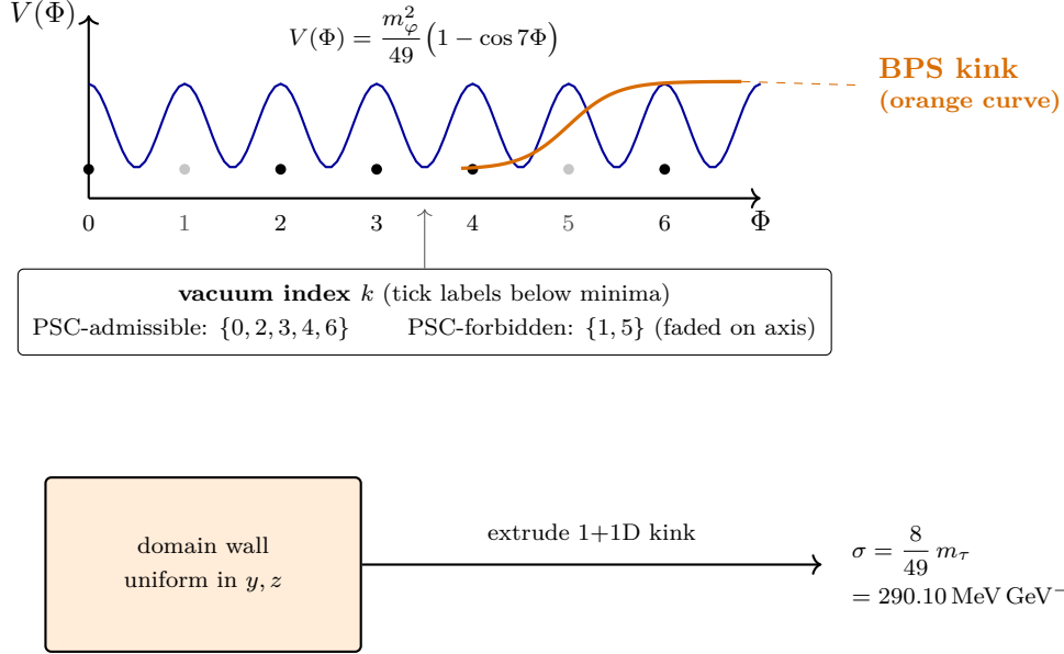
Figure 5.2: The \Phi_{\text{MDL}} potential has seven degenerate vacua at \Phi_k = 2\pi k/7 . Stable excitations are kinks in 1+1D (orange curve) and planar domain walls in 3+1D with the same BPS tension \sigma .
