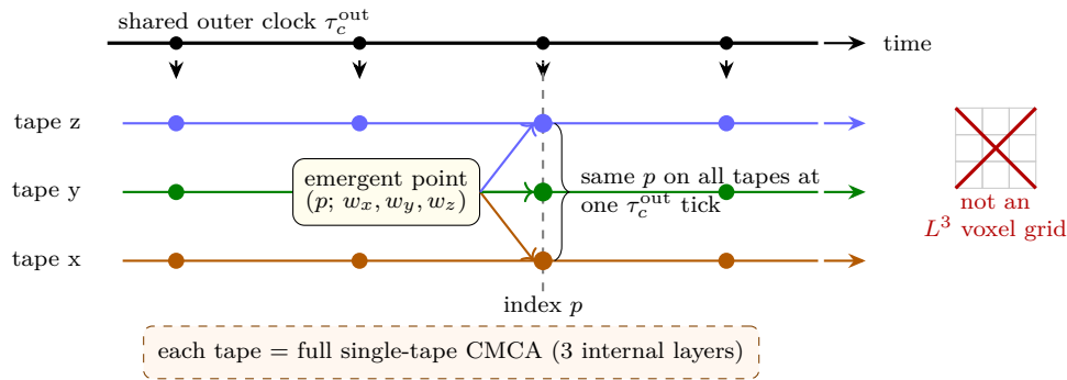
Figure 8.2: Three independent one-dimensional CMCA instances (rails) share one outer clock \tau_c^{\text{out}} . An emergent point in 3+1D is a synchronized triple of cell indices (p, p, p) at one clock tick, with winding readout (w_x, w_y, w_z) on the three tapes—not a cell in a three-dimensional lattice. A particle is a specific non-vacuum excitation of that structure (e.g. uniform triple (w, w, w) for SM states; see §6).
