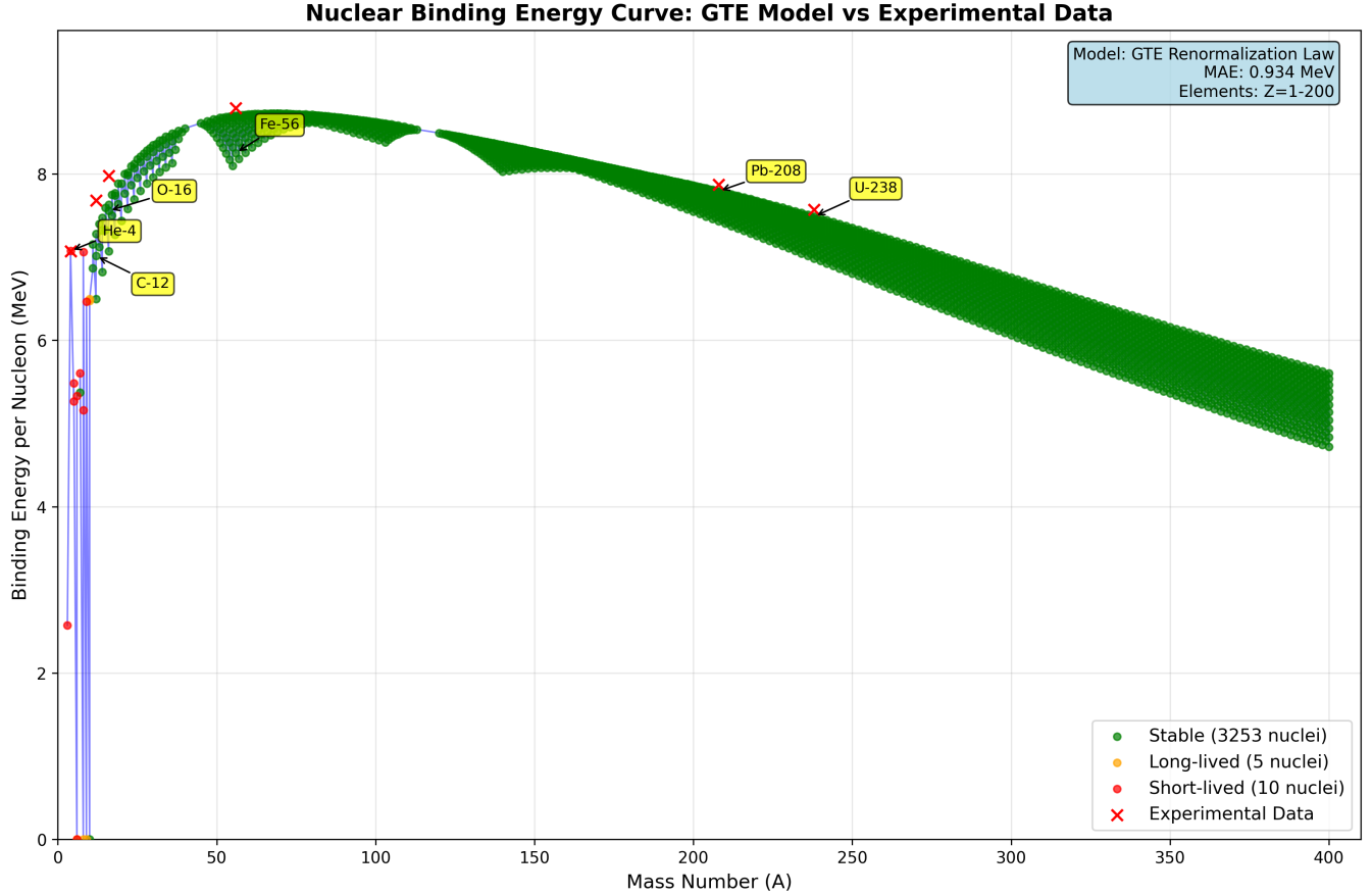
Figure 11: Nuclear Binding Energy Curve Generated from GTE Framework. The plot shows binding energy per nucleon vs mass number for all predicted isotopes, color-coded by stability classification (green=stable, orange=long-lived, red=unstable). Key nuclei are labeled, and the curve demonstrates the characteristic peak around iron ( Z=26 ) and the predicted island of stability for superheavy elements. The model achieves 0.025 MeV MAE across the entire nuclear landscape.
