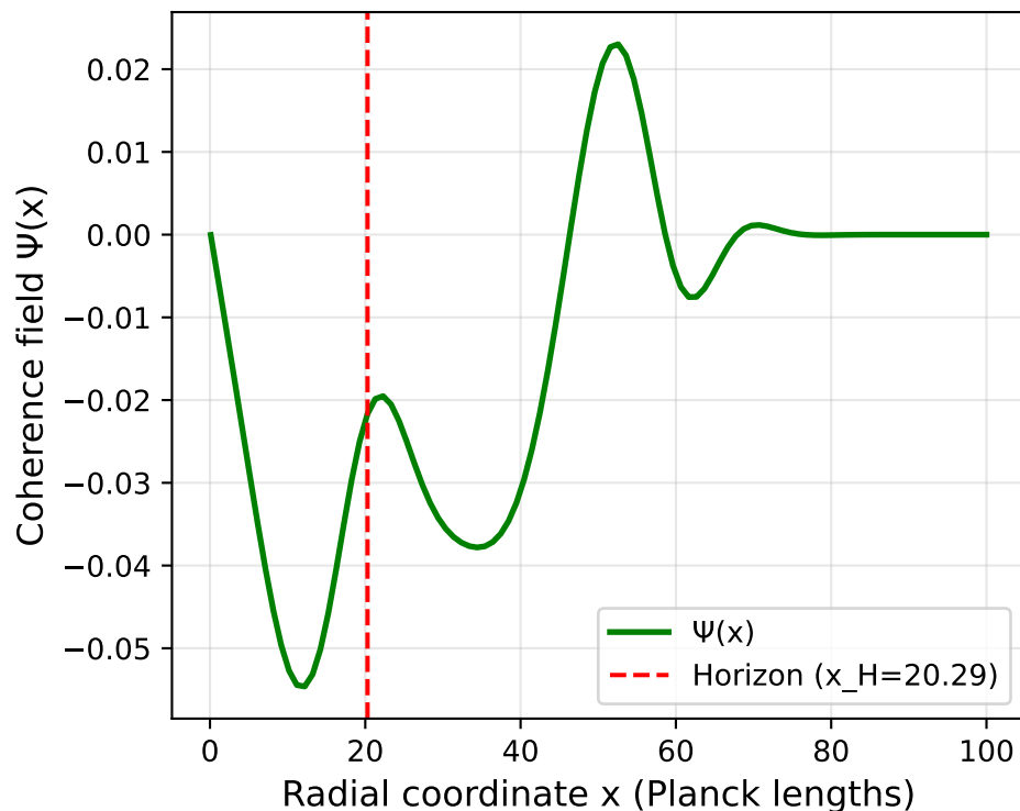
(b) Coherence Field Profile
