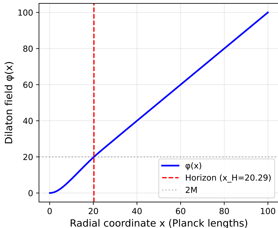
(a) Dilaton Field Profile
