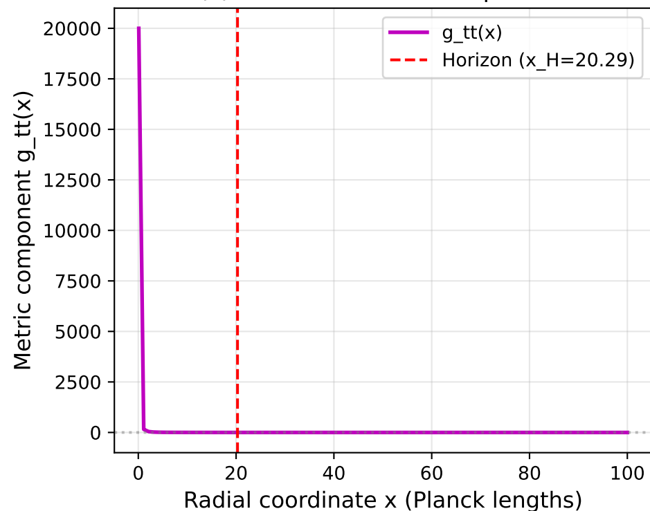
(c) Timelike Metric Component
