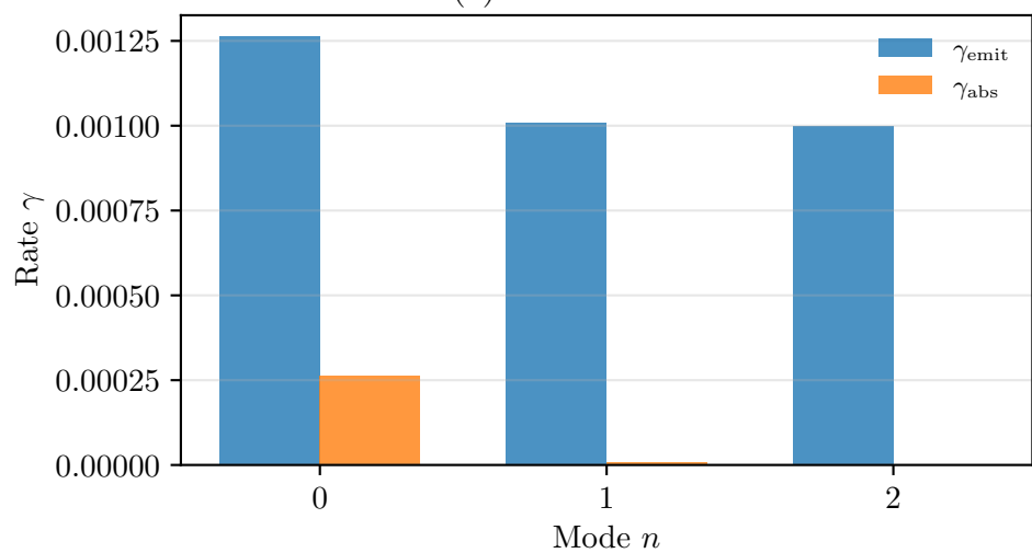
(e) Stinespring Dilation: GKSL \equiv Unitary
