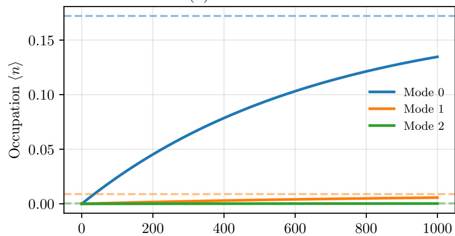
(c) Lindblad Rates
