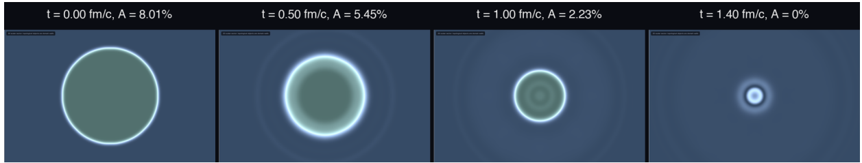
Figure 6.7: Direct empirical confirmation, in the 2+1D simulation, of the theorem's consequence for a nonzero-winding configuration: it cannot be a stable compact object. A single, genuinely one-elementary-kink-wide domain of down-type-quark vacuum ( w = 6 ) is seeded as an isolated disk (initial area fraction A = 8.01\% of the periodic domain) inside the vacuum background ( w = 0 ), then evolved under the pure-sector dynamics. The area fraction A (measured directly from the field, not read off a display) falls monotonically and completes a full collapse to A = 0 at t = 1.40 fm/c, matching a linear-in-time area-loss law characteristic of ordinary wall-tension-driven curvature flow, with no anomalous stability plateau. This is exactly what the no-go theorem above predicts: since a nonzero-winding configuration cannot be compact, an isolated nonzero-winding domain has no topological protection against ordinary curvature-driven collapse, and collapses completely, in contrast to the zero-winding, topologically-neutral breather solution of the pure-1+1D sector (analytic box above), which is provably non-radiating and persists indefinitely.
