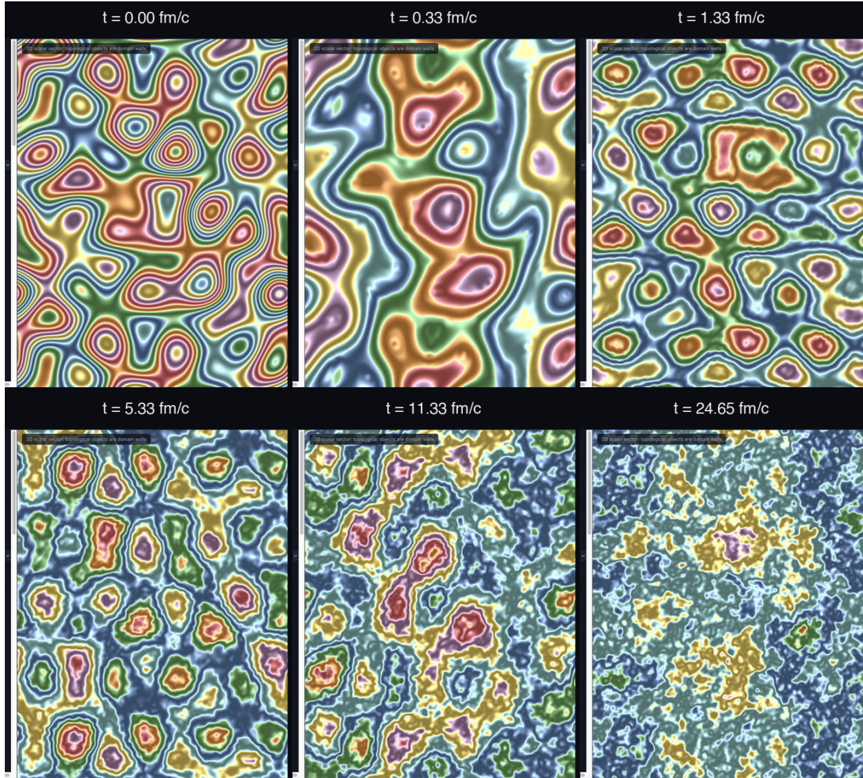
Figure 6.5: Pure-sector coarsening evolved from a genuinely random, unselected initial condition (the “random (self-organizing)” preset, seeded independently of Fig. 6.4’s curated eight-bubble setup), on the same 512^2 periodic grid. Panels, left to right, top to bottom: t = 0.00 fm/c (a fine-grained, unstructured mixture of all seven \mathbb{Z}_7 vacua); t = 0.33 , t = 1.33 , t = 5.33 , and t = 11.33 fm/c (curvature-driven merging coarsens the initial texture into progressively fewer and larger regions); t = 24.65 fm/c (advanced coarsening). Measuring the area fraction of each vacuum directly from the field at every panel: the vacuum sector ( w = 0 ) and the down-type-quark sector ( w = 6 ) grow monotonically from a combined 37.9% of the domain at t = 0 to 79.1% at t = 24.65 fm/c, while the three PSC-admissible charged sectors (up-type quarks w = 2 , W^+ /positron w = 3 , charged leptons w = 4 ) shrink from a combined 29.1% to 0.8%; the two PSC-forbidden dark-mirror sectors ( w = 1 , w = 5 ) hold a roughly steady \sim 20\% throughout. The same qualitative merging-and-shrinking behavior seen in Fig. 6.4’s curated setup therefore also proceeds from initial data with no imposed structure, confirming that curvature-driven coarsening is a property of the 2+1D dynamics itself rather than a feature specific to any particular starting configuration.
