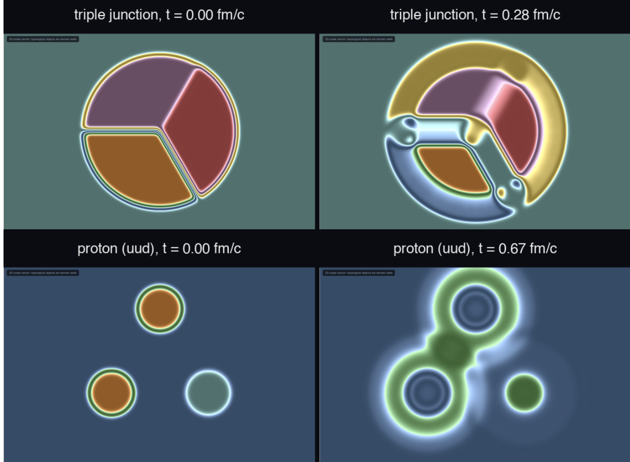
Figure 6.8: Two further 2+1D illustrations of the extended (never compact) character of \Phi_{\text{MDL}} winding-carrying configurations. Top row: the 2+1D analogue of the 3+1D triple-junction geometry analyzed in the Fock-space theorem below — three domains (up-type quarks w = 2 , orange; W^+ /positron w = 3 , red; charged leptons w = 4 , purple) meet at a point inside a down-type-quark ( w = 6 ) background; because the \mathbb{Z}_7 vacuum ring has no triangles, two of the three internal walls (2–3, 3–4) are single elementary kinks while the third (4–2) is an unavoidable composite two-step wall, visible here as the more strongly curved segment. By t = 0.28 \text{ fm}/c the three walls have evolved under tension in visibly different ways depending on this wall-order asymmetry. Bottom row: the illustrative “proton” preset — two up-type-quark domains and one down-type-quark domain, arranged with the charge-correct uud pattern ( Q = 2 \times \frac{2}{3} - \frac{1}{3} = +1 ) but not a derived bound state, since this pure- \Phi field has no colour/gauge confinement sector. By t = 0.67 \text{ fm}/c the two same-sector ( w = 2 ) domains have grown into each other and merged into one connected structure under ordinary wall-tension expansion (the same fast growth seen in Fig. 6.4), while the differently-sectored domain remains a separate, non-merging object — direct visual confirmation that nothing in the pure scalar dynamics binds the three domains together as a genuine composite particle.
