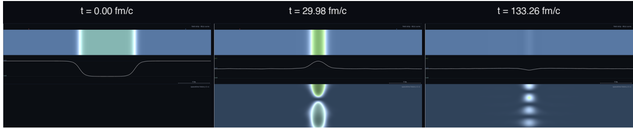
Figure 6.6: The qualitative annihilation-via-radiation mechanism, illustrated with the \mathbb{Z}_7 -degeneracy-preserving double-sine-Gordon proxy perturbation described above ( \eta = 0.05 ), contrasted directly with the pure-sector transmission of Fig. 6.3. A slow elementary antikink–kink pair is launched toward each other (initial positions x = \mp 10/m_\varphi , relative velocity 0.06c , below the capture threshold v \lesssim 0.10c stated above). Left: t = 0 , well separated, enclosing a one-step domain (teal). Middle: t \approx 30 fm/c, just after first contact — the pair has captured into an oscillating bound state (a bion): the spacetime-history strip below shows the two worldlines converging and wobbling around a common location instead of continuing past each other. Right: t \approx 133 fm/c — the bion has decayed almost completely by radiation (the discrete, shrinking “bead” pattern in the history strip is the outgoing radiation), the field strip has returned to a nearly featureless vacuum, and a direct count of elementary-kink crossings in the field is exactly zero: the pair has genuinely annihilated, while total field energy remains conserved to 1 \times 10^{-4} relative (verified directly from the simulation, not merely read off the display), confirming the energy went into propagating radiation rather than leaving the system. This is the opposite qualitative outcome from Fig. 6.3’s clean elastic pass-through, and is exactly the capture/annihilation phenomenology the boxed sine-Gordon result above proves is absent in the pure sector but present once integrability is broken.
