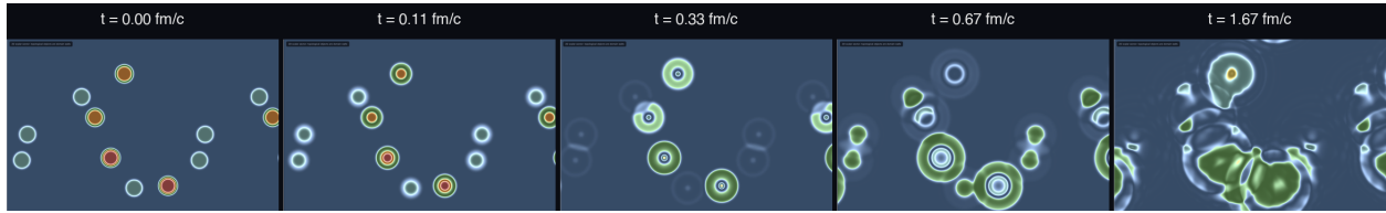
Figure 6.4: The many-body richness of the pure sector, generalized to 2+1D: eight non-overlapping circular domains are seeded on a periodic 512^2 grid, each randomly assigned one of the four PSC-admissible elementary sectors (orange = up-type quarks, w=2 ; red = W^+ /positron, w=3 ; purple = charged leptons, w=4 ; grey-teal = down-type quarks, w=6 ), and evolved under the same leapfrog integrator as Fig. 6.3, still in the exactly-integrable pure sector. Panels, left to right, same run: t = 0 (eight separate domains); t = 0.11 fm/c; t = 0.33 fm/c; t = 0.67 fm/c; t = 1.67 fm/c (several domains have merged into connected structures, and same-sector domains that meet no longer have a wall between them). Important caveat, distinct from the exact 1+1D result above: unlike the true 1+1D solitons of Fig. 6.3, a curved domain wall in 2+1D is not topologically protected against curvature-driven wall tension — integrability is a strictly 1+1D phenomenon (§6.5 below makes this precise). The rapid growth and merging visible here is exactly this tension-driven curvature flow, not a 1+1D-style elastic collision; it is nonetheless a direct, honest rendering of the same certified \Phi_{\text{MDL}} Lagrangian’s dynamics one dimension higher, and it is the qualitative behavior that motivates the quantitative single-bubble decay measurement of Fig. 6.7 below.
