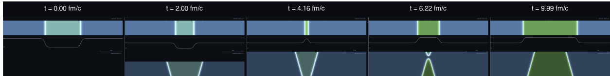
Figure 6.3: Direct leapfrog integration of an elementary kink–antikink pair in the pure \mathbb{Z}_7 sector, reproducing the exact two-soliton solution \Phi_{\text{KA}}(x, t) of Eq. (6.5)’s box above. A single elementary antikink (initial position x = -15/m_\varphi , velocity +0.4c ) and a single elementary kink (initial position x = +15/m_\varphi , velocity -0.4c ) approach, overlap, and separate. Panels, left to right: t = 0 (well separated, enclosing a one-step \mathbb{Z}_7 domain, teal); t = 2.00 fm/c (approaching); t = 4.16 fm/c (maximal overlap — the field strip shows a single smooth bump, the classic sine-Gordon collision profile, with no radiation emitted); t = 6.22 fm/c (just after crossing — the enclosed domain has flipped color, showing the two solitons have passed through rather than annihilated); t = 9.99 fm/c (well separated again, having swapped sides). The lower strip in each panel is the scrolling spacetime-history (worldline) plot; the clean “X” crossing pattern is the signature of elastic, radiation-free transmission — there is no capture, no bion formation, and no annihilation, exactly as the exact solution and the many-kink-gas simulation below both predict for the pure sector. An interactive, live version of this simulation is linked in the footnote at this section’s opening.
