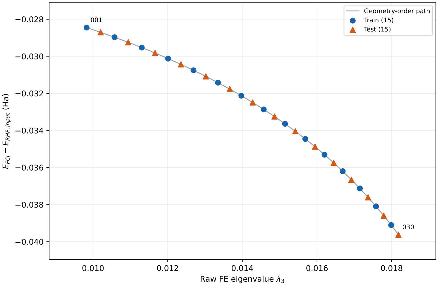
BeH2 · column 3 · correlation energy vs active FE
