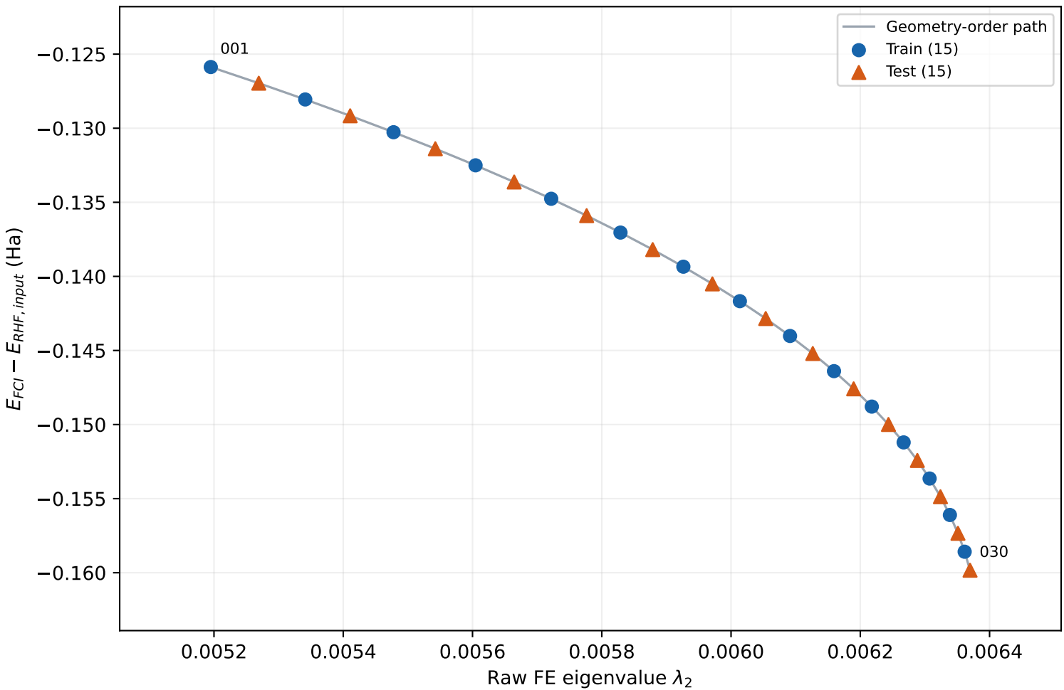
CO · column 2 · correlation energy vs active FE
