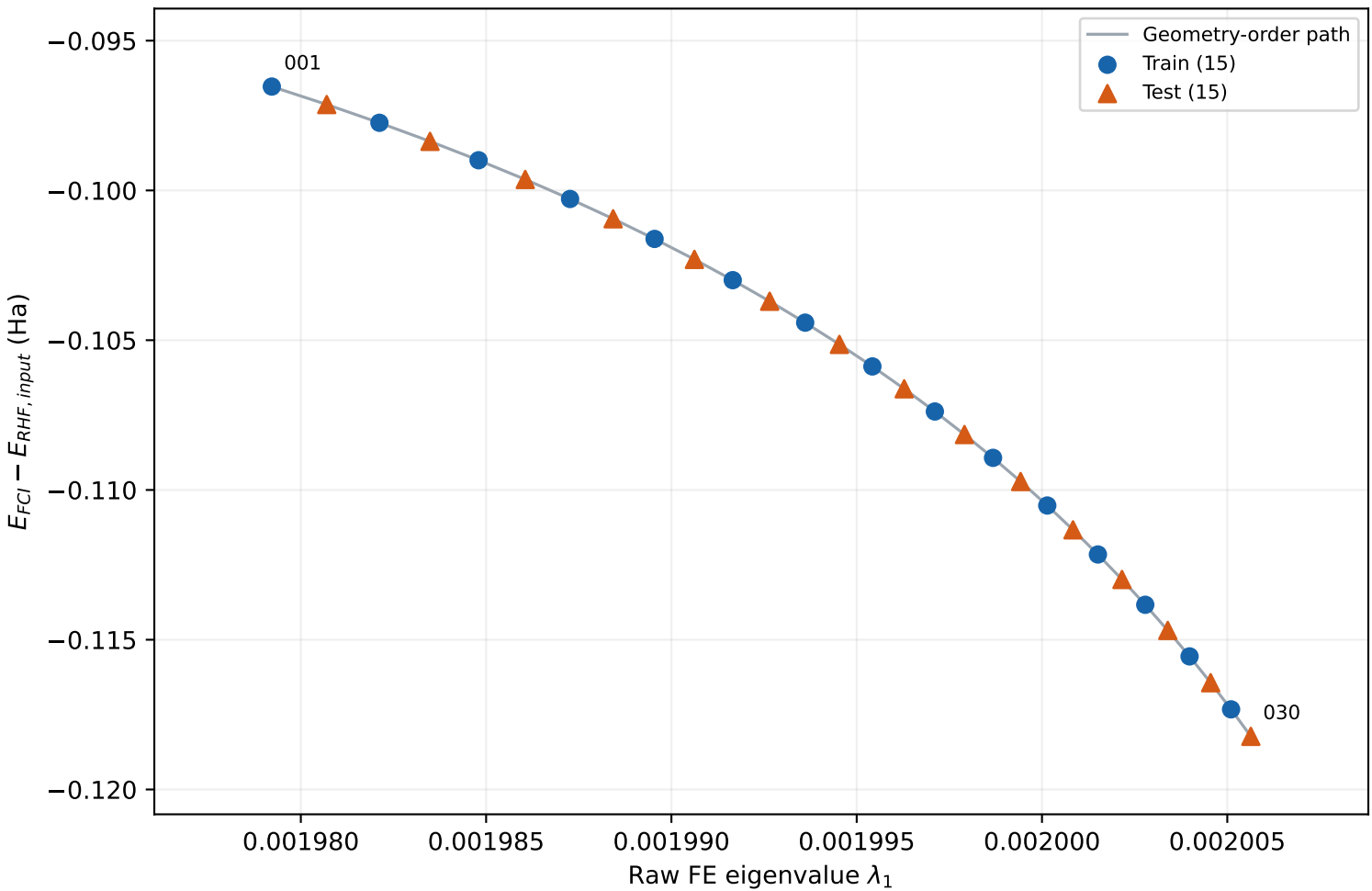
H2O2 · column 1 · correlation energy vs active FE
