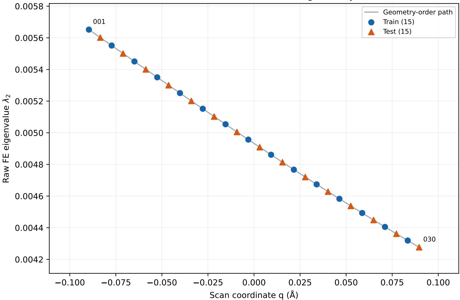
H2O2 · column 2 · active FE vs geometry
