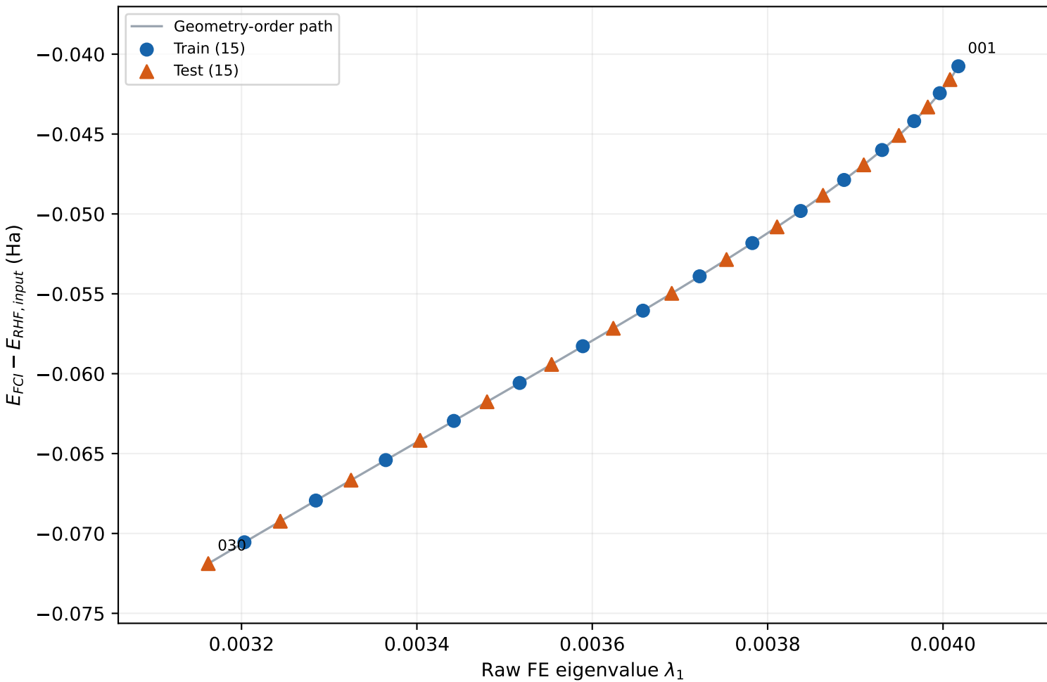
H2O · column 1 · correlation energy vs active FE
