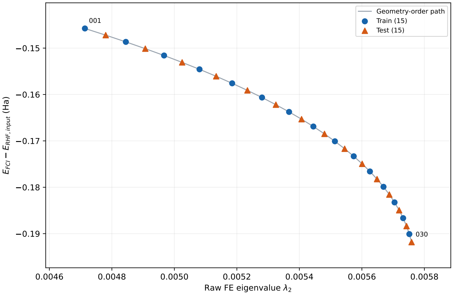
N2 · column 2 · correlation energy vs active FE
