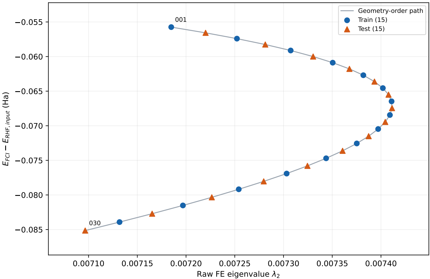
NH3 · column 2 · correlation energy vs active FE
