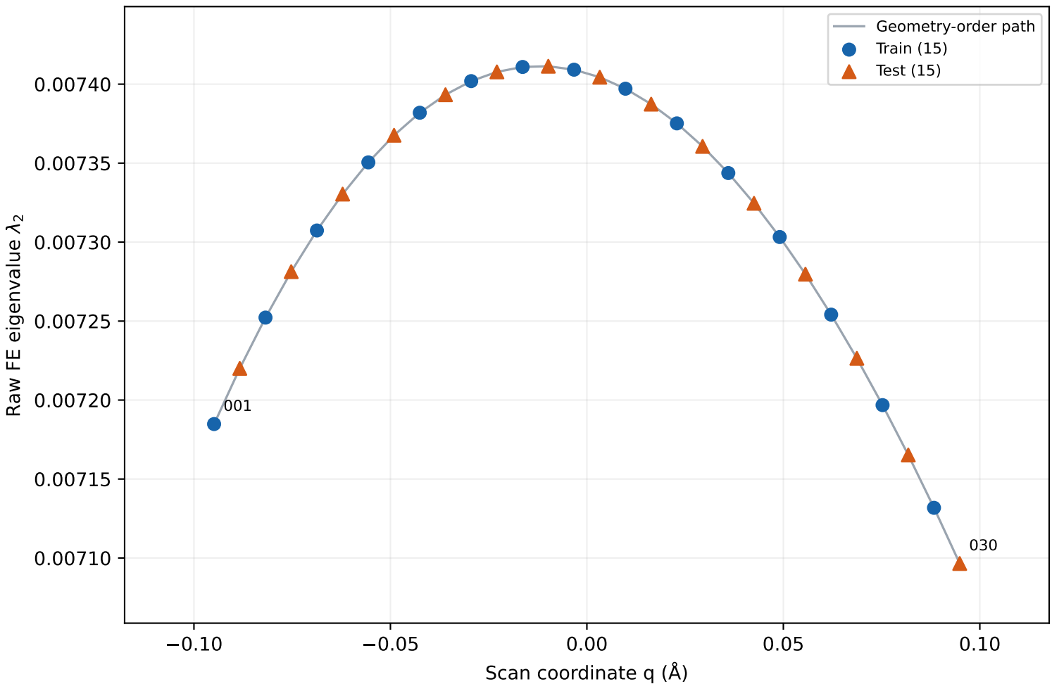
NH3 · column 2 · active FE vs geometry
