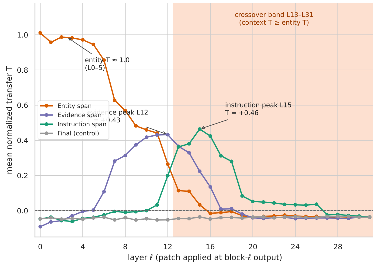
(a) Entity-state layer sweep: normalized transfer by span
