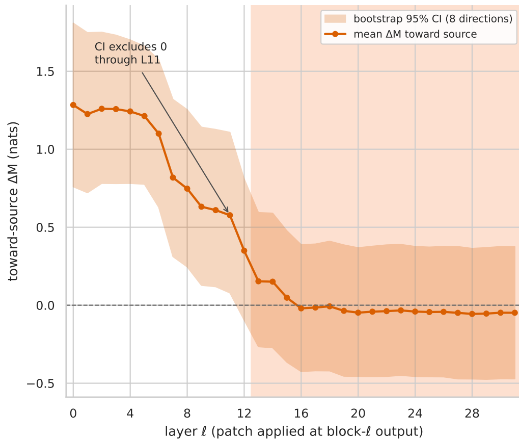
(b) Entity-span sufficiency: toward-source \Delta M
